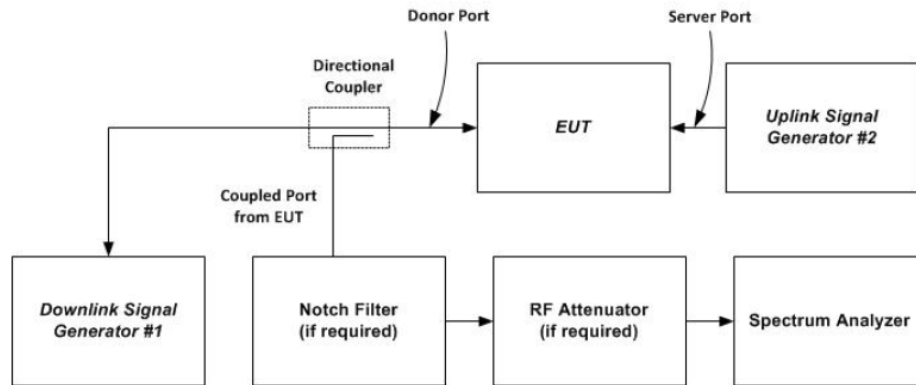
Figure 5 – Variable gain instrumentation test setup
