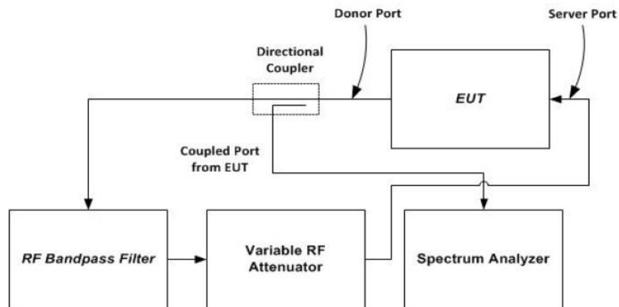
Figure 7 – Oscillation detection instrumentation test setup
