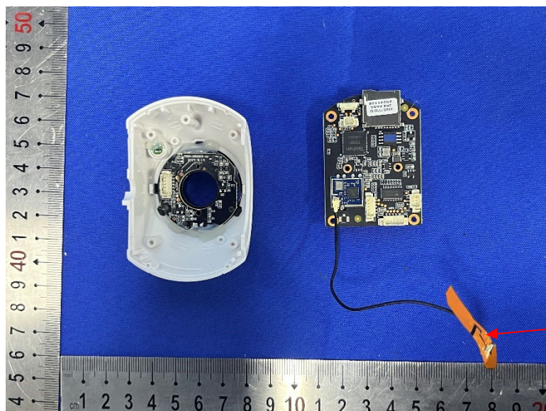
WIFI Antenna
