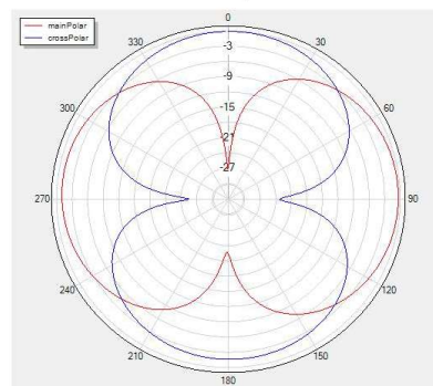
Theta=90 freq=5300MHz
