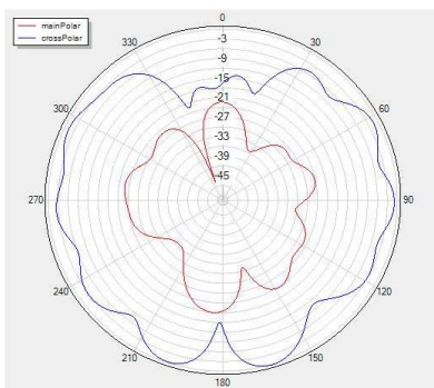
Phi=0 freq=5300MHz
