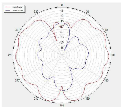
Phi=90 freq=5300MHz
