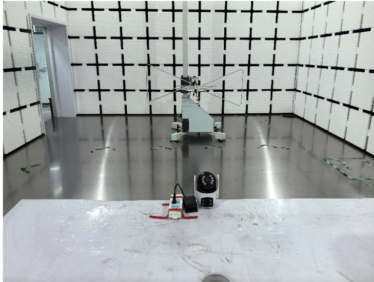
Radiated Emission
