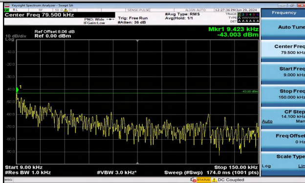
Band2_10MHz_QPSK_19150_1RB#0_0.009~0.15_0.009 ~0.15
