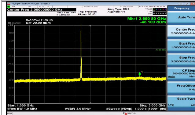
Band2_5MHz_16QAM_18900_1RB#0_1000~3000_1000~3000
