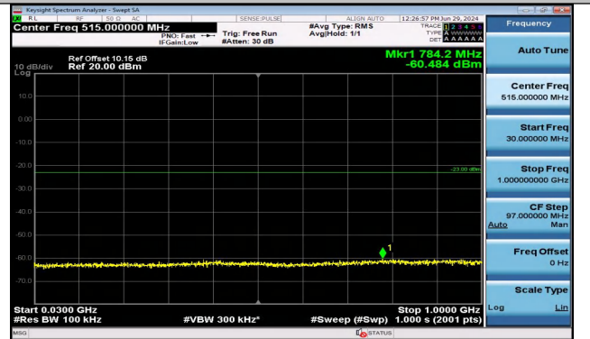
Band2_10MHz_16QAM_18900_1RB#0_30~1000_30~100 0
