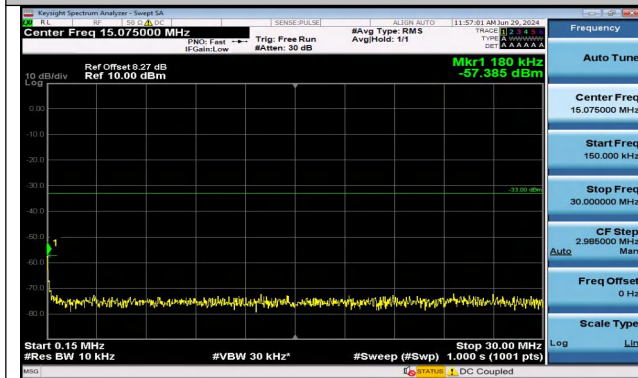
Band2_5MHz_16QAM_18900_1RB#0_0.15~30_0.15~30
