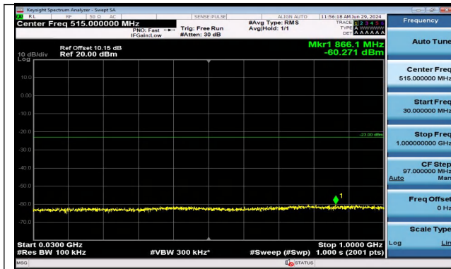
Band2_5MHz_QPSK_18900_1RB#0_30~1000_30~1000
