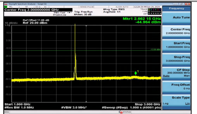
Band2_10MHz_QPSK_18650_1RB#0_1000~3000_1000~3000 000
