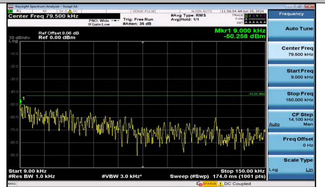
Band2_5MHz_16QAM_18900_1RB#0_0.009~0.15_0.009~0.15
