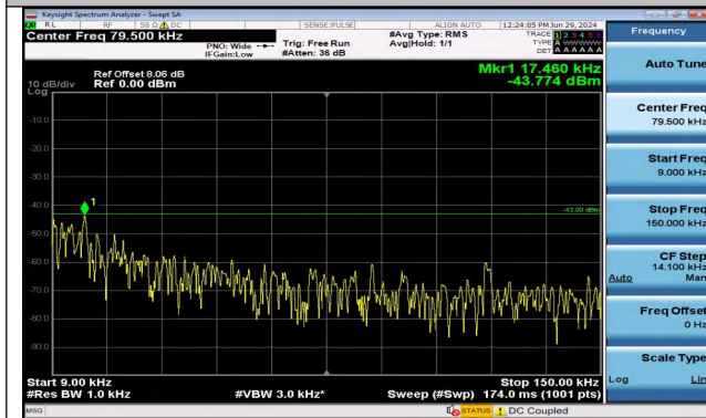
Band2_10MHz_QPSK_18650_1RB#0_0.009~0.15_0.009 ~0.15
