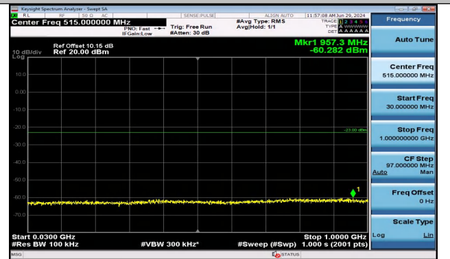
Band2_5MHz_16QAM_18900_1RB#0_30~1000_30~1000
