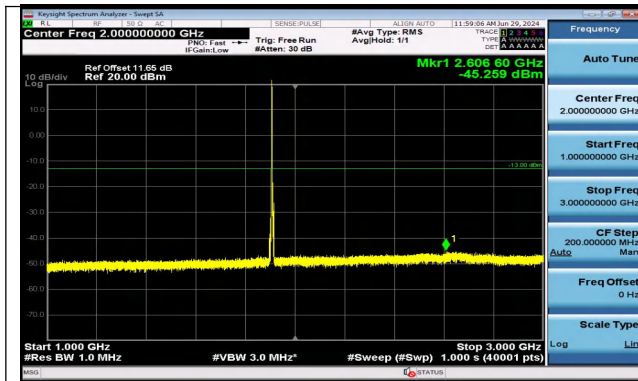
Band2_5MHz_16QAM_19175_1RB#0_1000~3000_1000 ~3000
