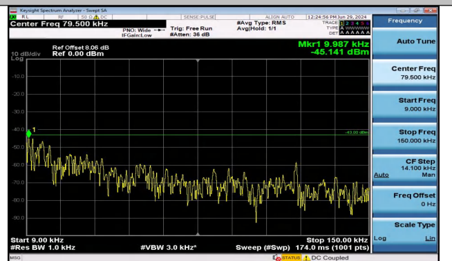
Band2_10MHz_16QAM_18650_1RB#0_0.009~0.15_0.009 ~0.15
