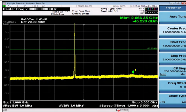
Band2_10MHz_16QAM_18900_1RB#0_1000~3000_1000 ~3000
