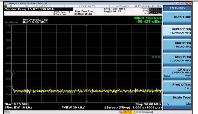
Band2_10MHz_QPSK_19150_1RB#0_0.15~30_0.15~30
