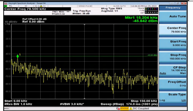
Band2_10MHz_16QAM_18900_1RB#0_0.009~0.15_0.009 ~0.15
