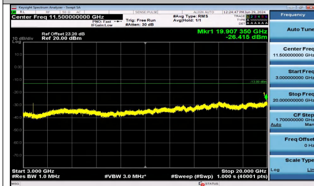
Band2_10MHz_QPSK_18650_1RB#0_3000~20000_3000 ~20000
