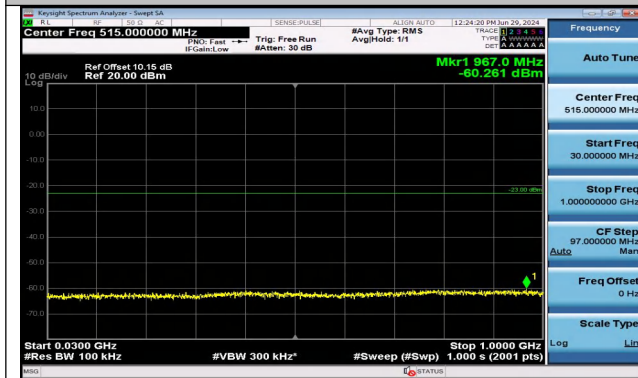
Band2_10MHz_QPSK_18650_1RB#0_30~1000_30~1000 000
