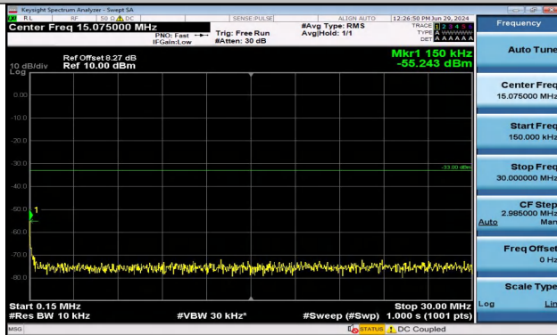
Band2_10MHz_16QAM_18900_1RB#0_0.15~30_0.15~3 0
