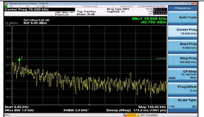
Band2_15MHz_16QAM_18675_1RB#0_0.009~0.15_0.009 ~0.15
