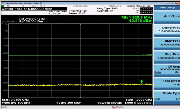
Band2_15MHz_QPSK_18675_1RB#0_30~1000_30~1000
