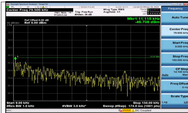
Band2_15MHz_QPSK_18675_1RB#0_0.009~0.15_0.009 ~0.15
