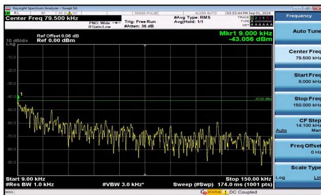
Band2_15MHz_QPSK_18900_1RB#0_0.009~0.15_0.009 ~0.15
