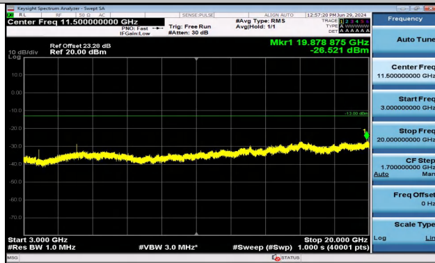
Band2_15MHz_QPSK_18900_1RB#0_3000~20000_3000
