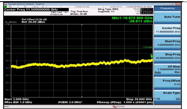
Band2_15MHz_16QAM_18675_1RB#0_3000~20000_3000 ~20000
