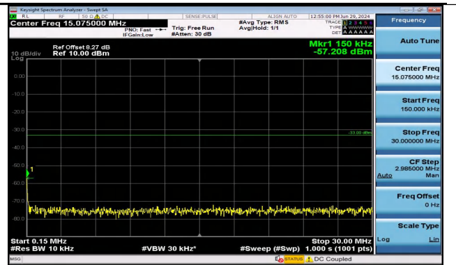
Band2_15MHz_QPSK_18675_1RB#0_0.15~30_0.15~30
