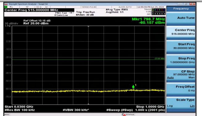
Band2_15MHz_16QAM_18675_1RB#0_30~1000_30~1000 0
