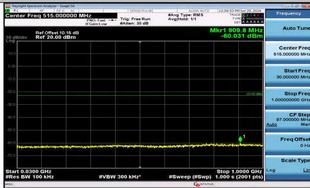
Band2_15MHz_QPSK_18900_1RB#0_30~1000_30~1000
