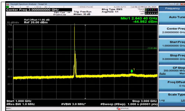
Band2_15MHz_16QAM_18675_1RB#0_1000~3000_1000 ~3000
