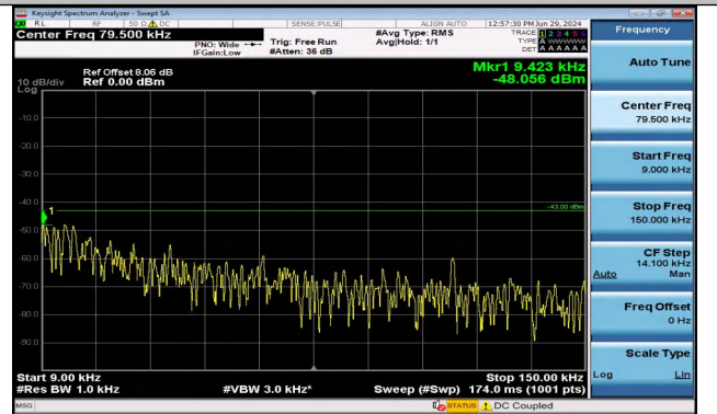
Band2_15MHz_16QAM_18900_1RB#0_0.009~0.15_0.009
