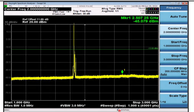
Band2_15MHz_QPSK_18675_1RB#0_1000~3000_1000~3000
