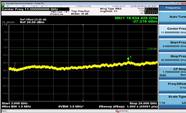
Band2_15MHz_QPSK_18675_1RB#0_3000~20000_3000~20000
