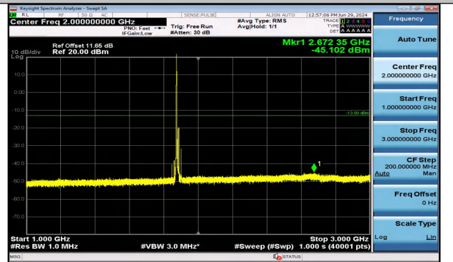
Band2_15MHz_QPSK_18900_1RB#0_1000~3000_1000~3000
