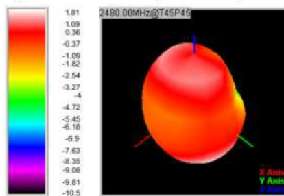
© 3D Gain Pattern (2480 MHz)
