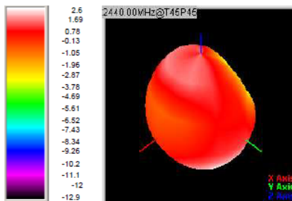
© 3D Gain Pattern (2440 MHz)
