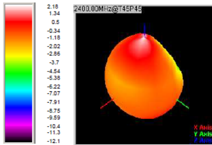
© 3D Gain Pattern (2400 MHz)
