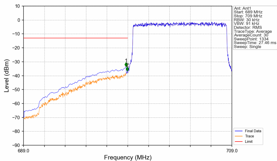
Band12_10MHz_QPSK_LCH_704MHz_RB_50_0_NTNV
