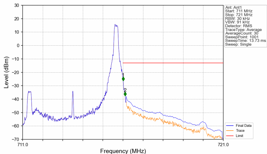
Band12_5MHz_QPSK_HCH_713.5MHz_RB_1_24 NTN
