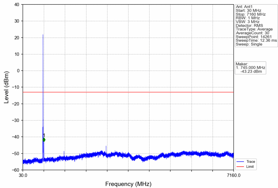
Band12_5MHz_QPSK_HCH_713.5MHz_RB_1_24 NTN
