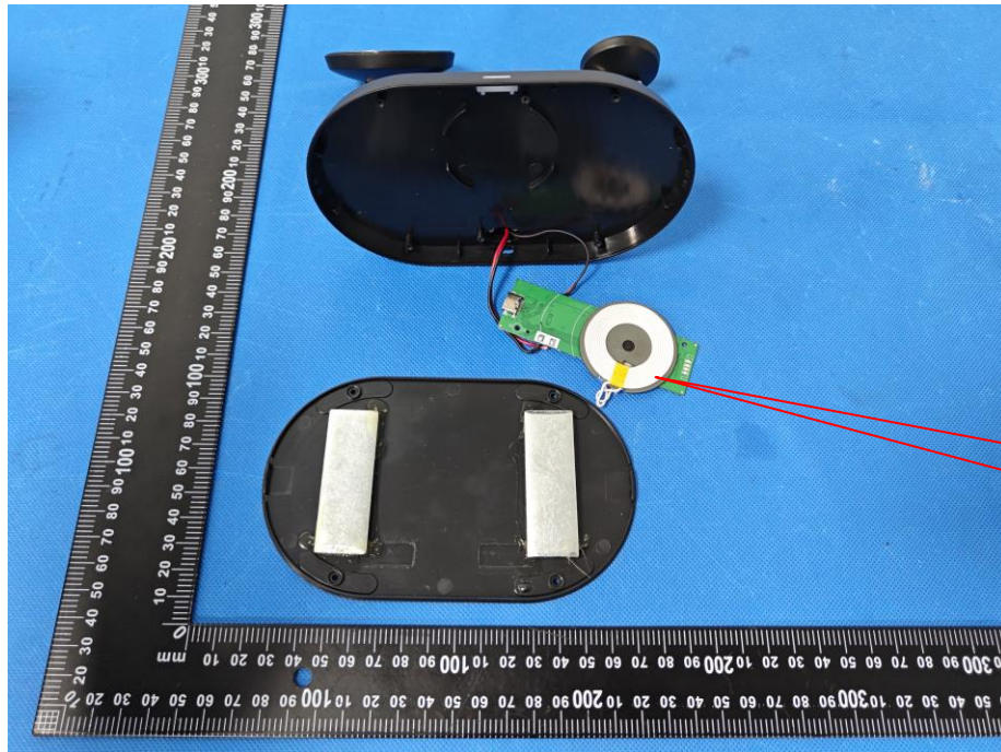
Antenna Earphone
