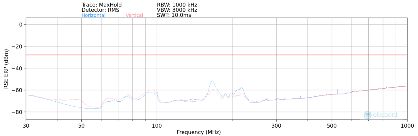
Plot 6-17. Radiated Spurious Plot (C-V2X RSU) (30MHz – 1GHz)
