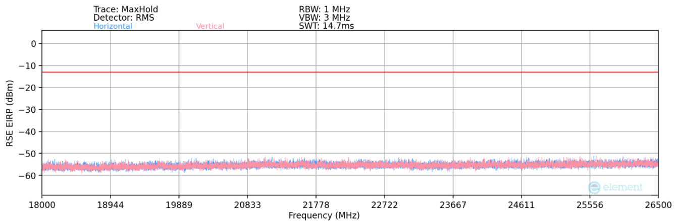
Plot 6-23. Radiated Spurious Plot (C-V2X RSU – LTE BAND 5)
