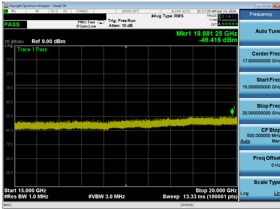
Plot 6-12. Conducted Spurious Plot (C-V2X RSU)
