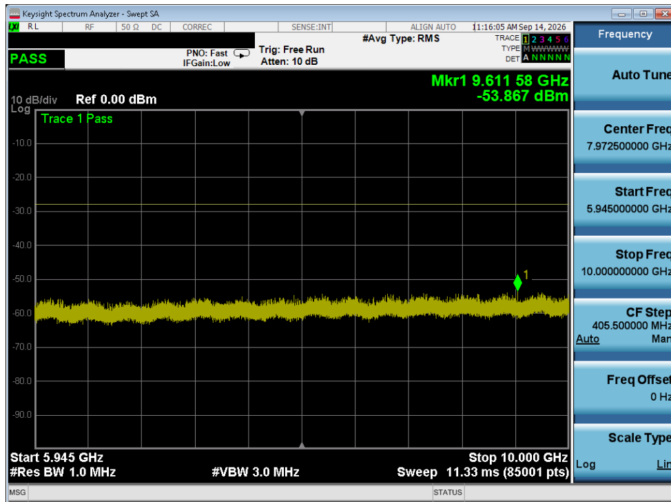
Plot 6-10. Conducted Spurious Plot (C-V2X RSU)
