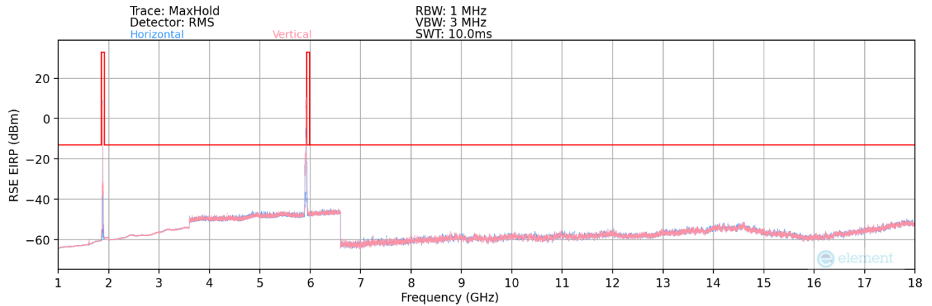
Plot 6-26. Radiated Spurious Plot (C-V2X RSU – LTE BAND 2)
