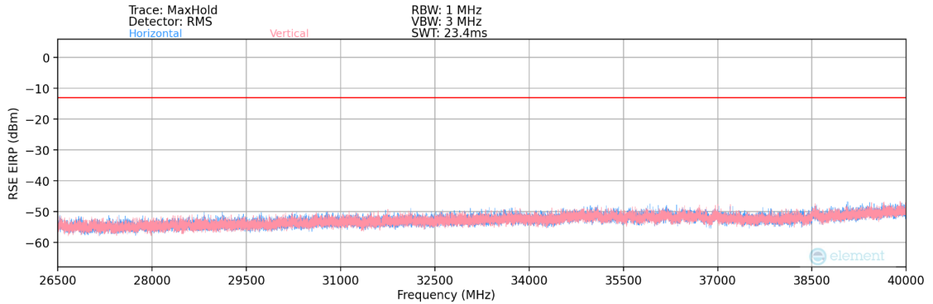
Plot 6-28. Radiated Spurious Plot (C-V2X RSU – LTE BAND 2)
