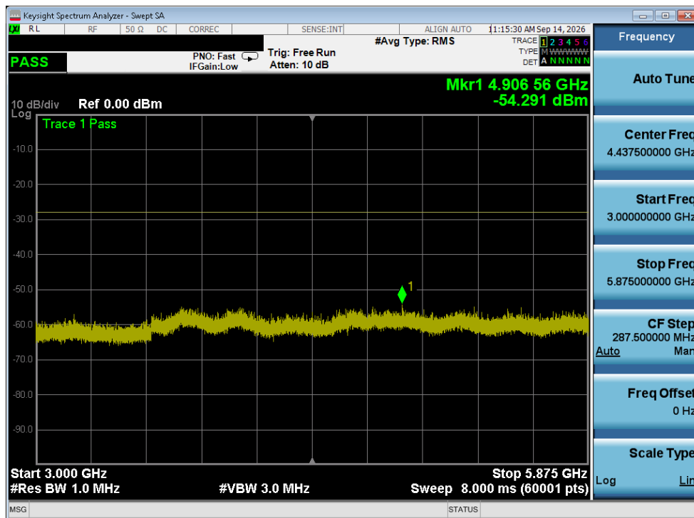
Plot 6-9. Conducted Spurious Plot (C-V2X RSU)
