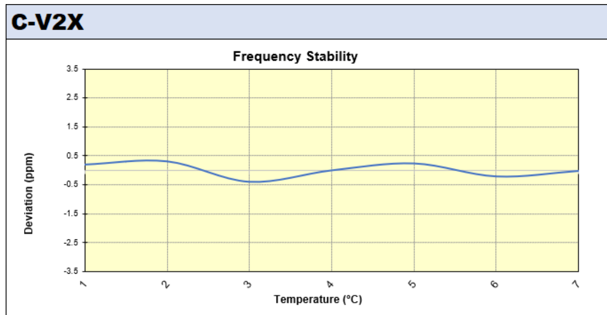
Plot 6-29. Frequency Stability Chart (C-V2X RSU)
