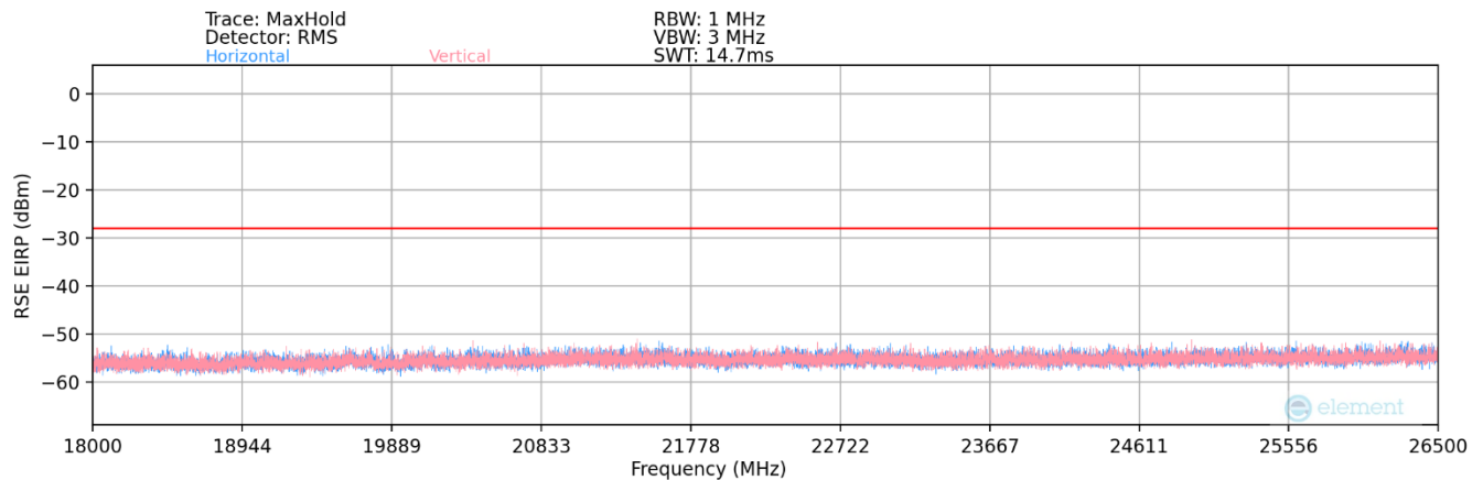
Plot 6-19. Radiated Spurious Plot (C-V2X RSU) (18GHz – 26.5GHz)
