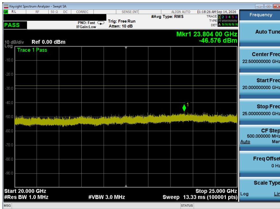
Plot 6-13. Conducted Spurious Plot (C-V2X RSU)
