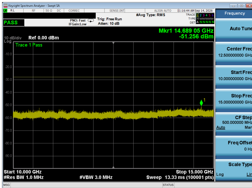
Plot 6-11. Conducted Spurious Plot (C-V2X RSU)
