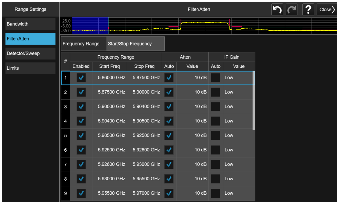
Plot 6-5. Out of Band Emissions Settings
