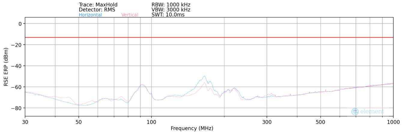
Plot 6-25. Radiated Spurious Plot (C-V2X RSU – LTE BAND 2)
