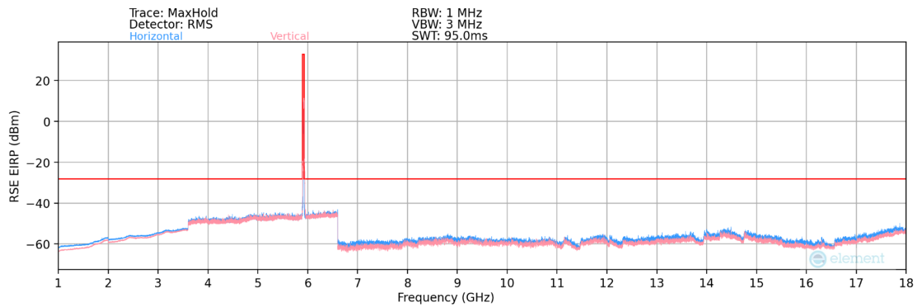
Plot 6-18. Radiated Spurious Plot (C-V2X RSU) (1GHz – 18GHz)
