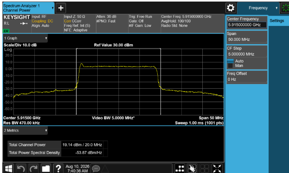
Plot 6-1. Conducted Output Power Plot (C-V2X RSU)
