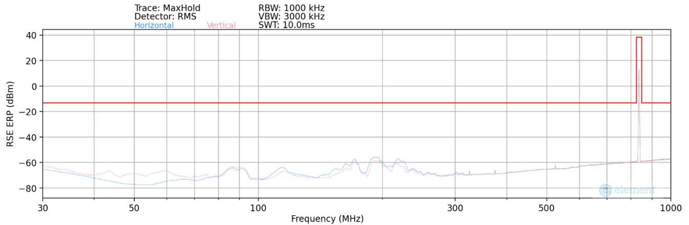
Plot 6-21. Radiated Spurious Plot (C-V2X RSU – LTE BAND 5)
