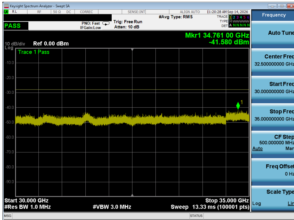
Plot 6-15. Conducted Spurious Plot (C-V2X RSU)
