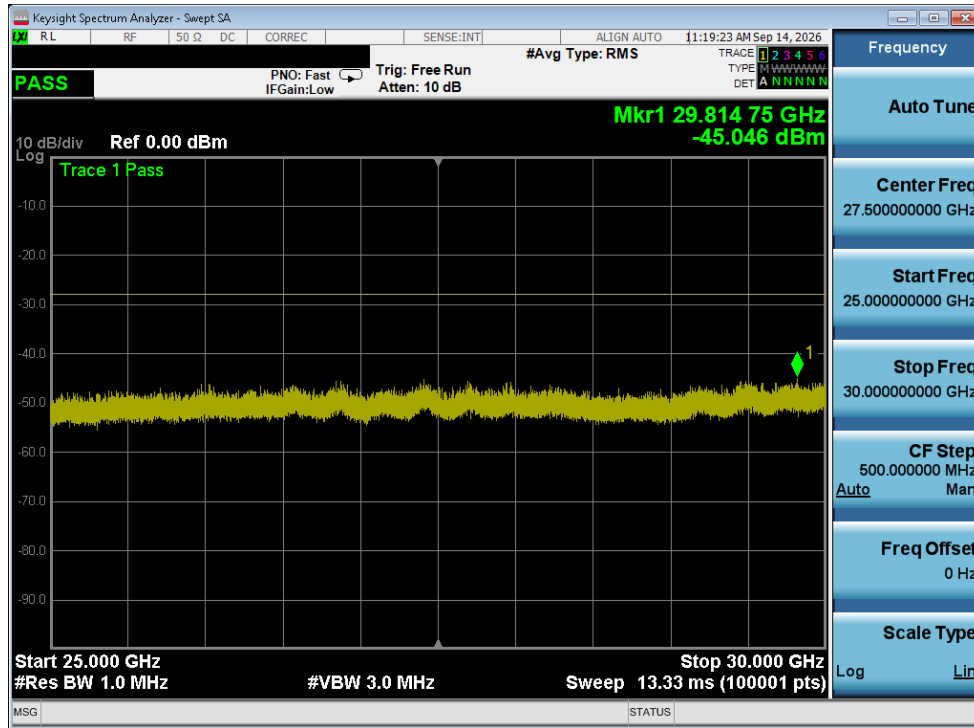
Plot 6-14. Conducted Spurious Plot (C-V2X RSU)
