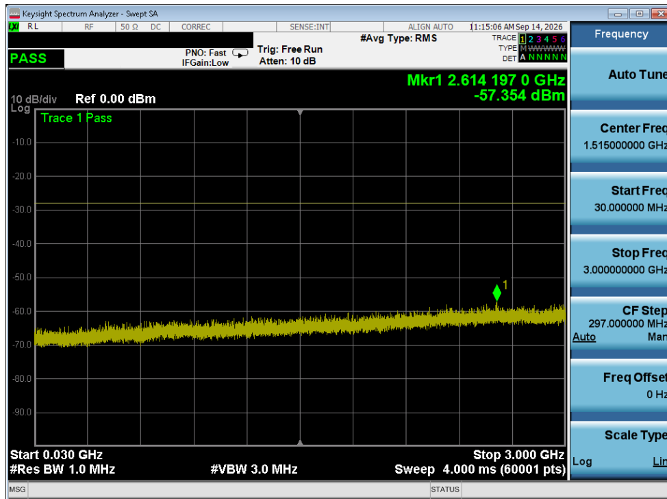
Plot 6-8. Conducted Spurious Plot (C-V2X RSU)
