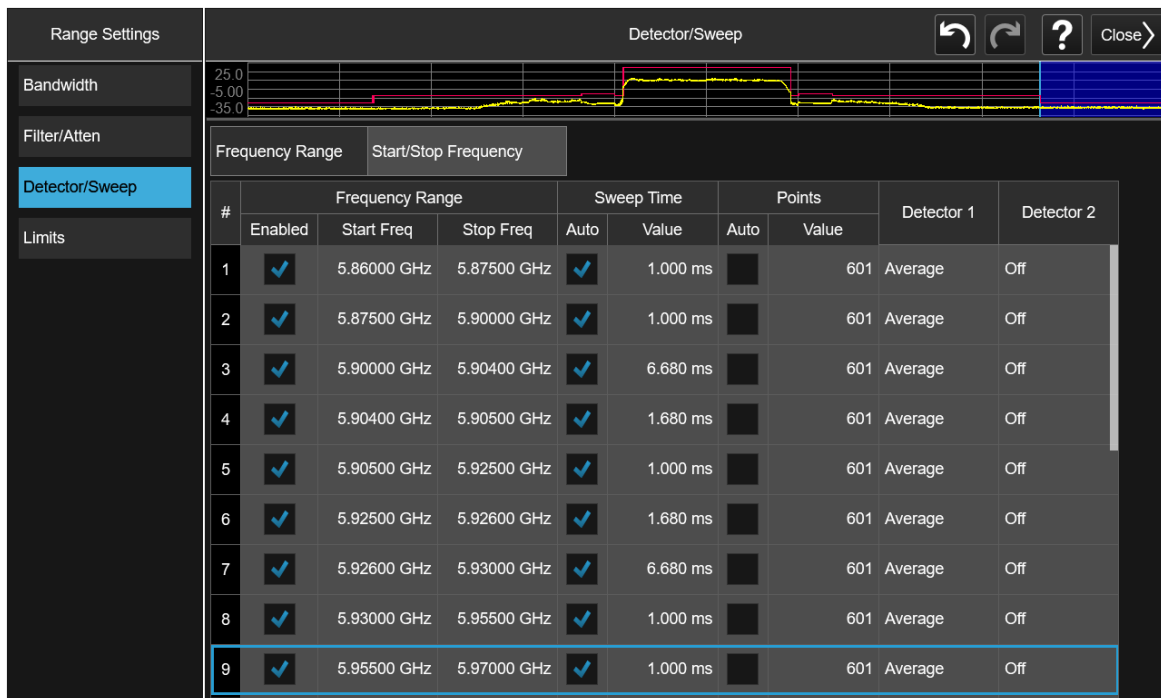
Plot 6-6. Out of Band Emissions Settings
