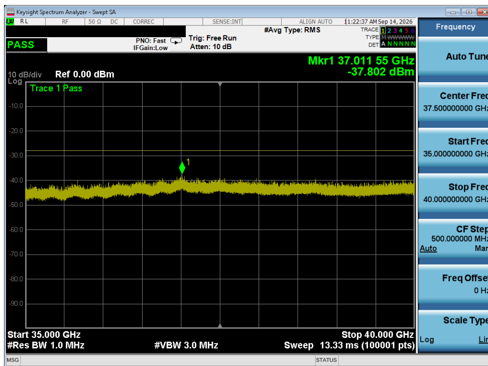
Plot 6-16. Conducted Spurious Plot (C-V2X RSU)
