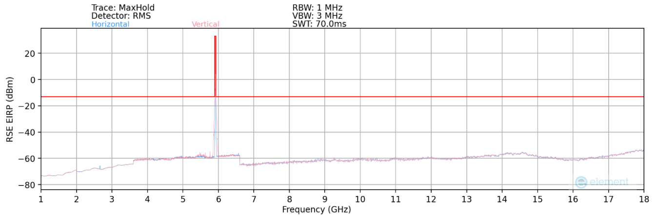
Plot 6-22. Radiated Spurious Plot (C-V2X RSU – LTE BAND 5)
