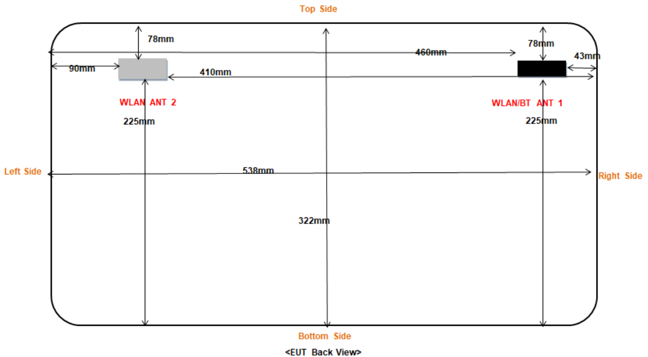
Fig 7.2 Block Diagram for EUT Antenna Position EUT Sizes: Long 538mm; width:322mm; height:48mm
