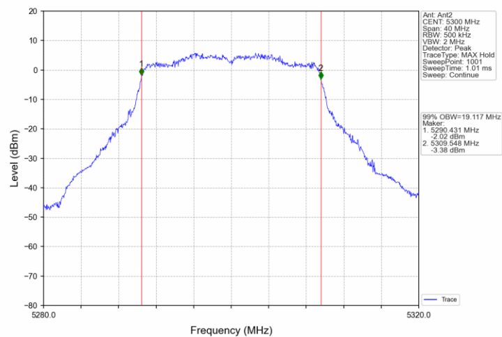
802.11ax(HEW20)_MCH_5300MHz_Ant2_NTNV
