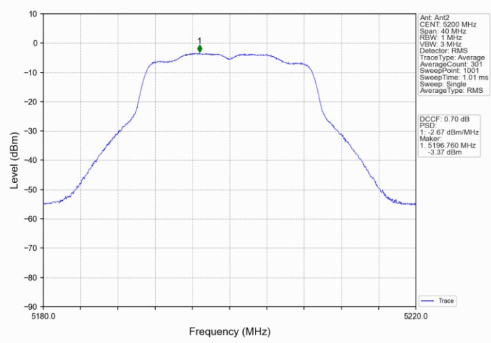
802.11ac(VHT20)_MCH_5200MHz_MIMO_NTNV
