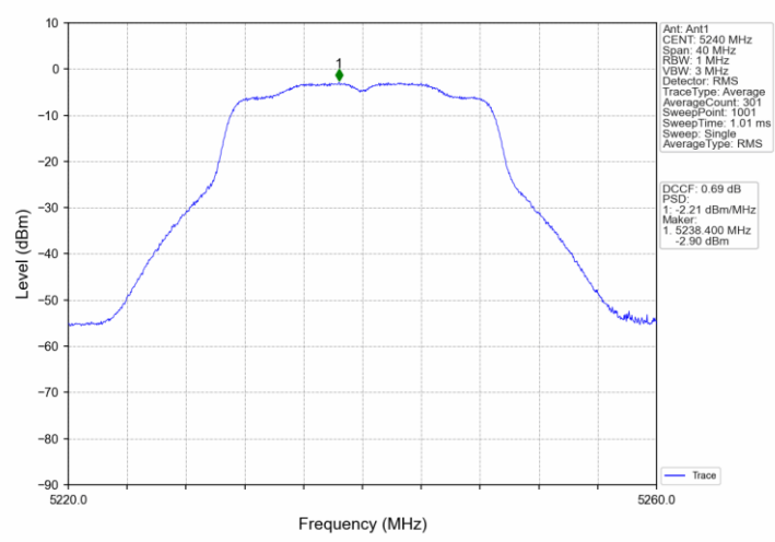
802.11ac(VHT20)_HCH_5240MHz_Ant1_NTNV
