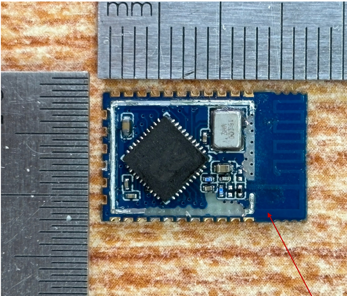
PCB on board antenna location
