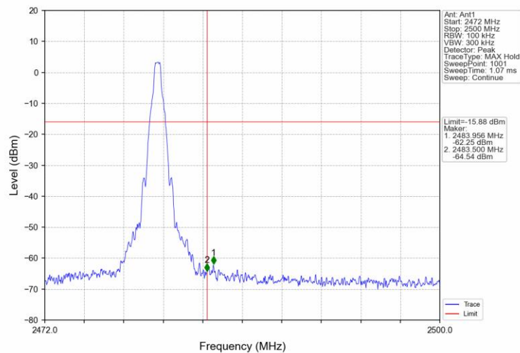
GFSK_DH5_HCH_2480MHz_Ant_1_NTNV
