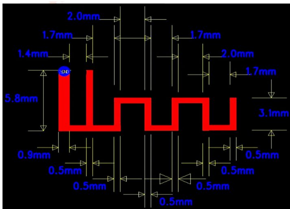
Antenna Photo &amp; Length(mm)
