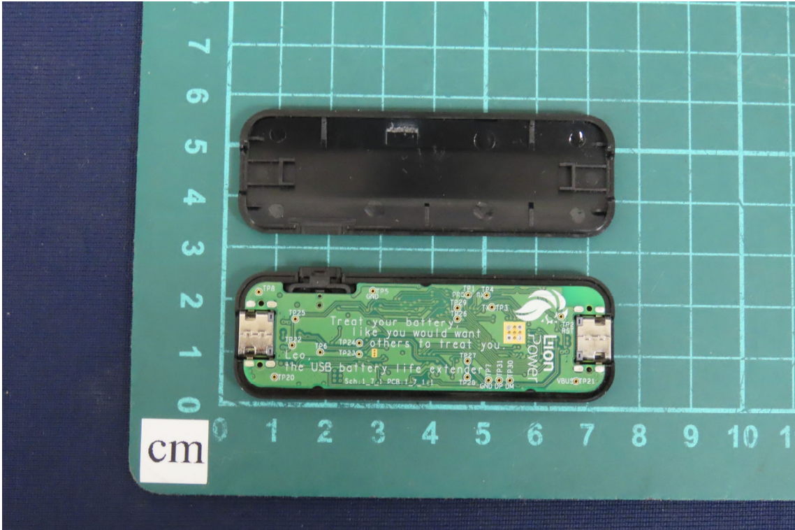
(1) EUT Photo
