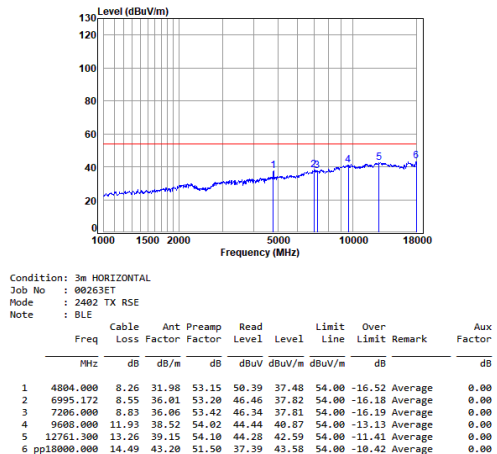
BLE_1M_TX_CH_00_Horizontal-Avg
