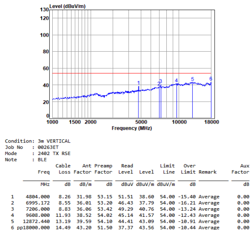
BLE_1M_TX_CH_00_Vertical-Avg
