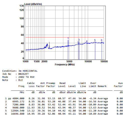
BLE_1M_TX_CH_00_Horizontal-Avg
