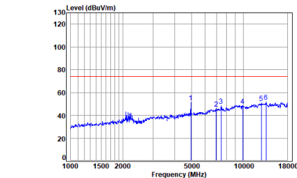
BLE_1M_TX_CH_39_Vertical-Peak
