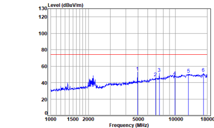
BLE_1M_TX_CH_39_Horizontal-Peak
