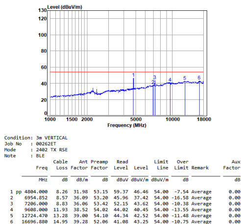
BLE_1M_TX_CH_00_Vertical-Avg
