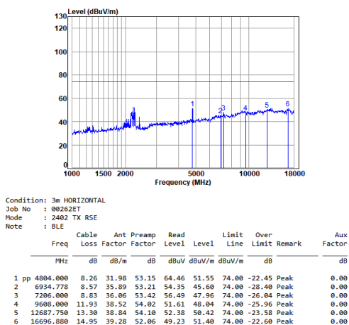
BLE_1M_TX_CH_00_Horizontal-Peak
