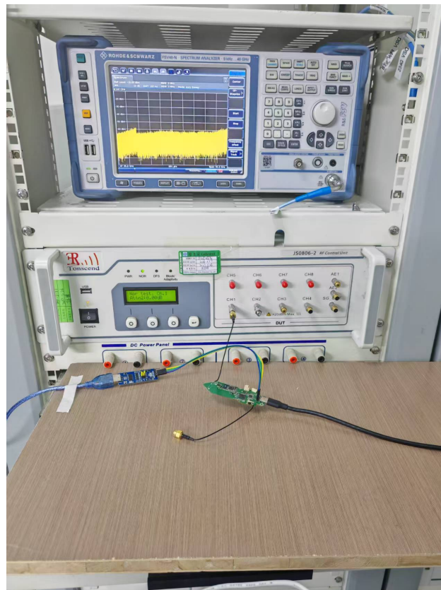
Photograph 3: Set-up photo for Conducted emission test
