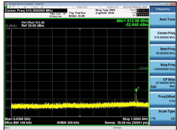
11N20SISO-Ant1-2412-30~1000-PASS
