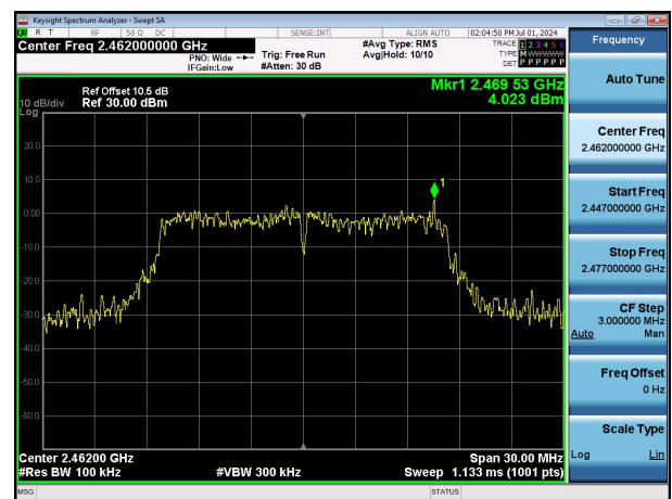
11G-Ant1-2462-0~Reference-PASS
