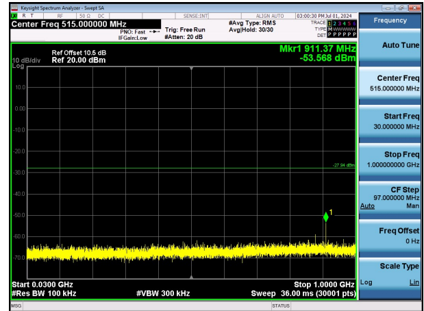
11N20SISO-Ant1-2462-30~1000-PASS
