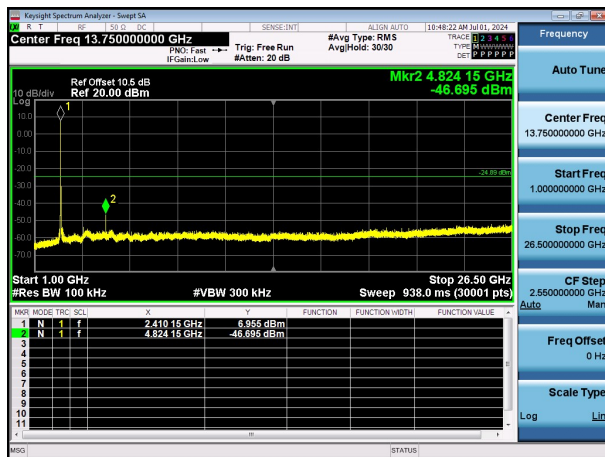
11B-Ant1-2412-1000~26500-PASS
