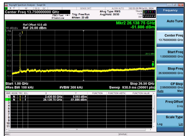
11N20SISO-Ant1-2437-1000~26500-PASS
