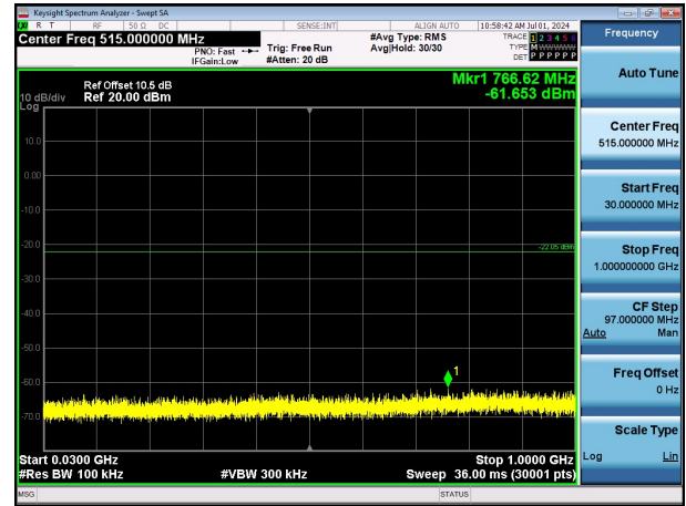
11B-Ant1-2462-30~1000-PASS
