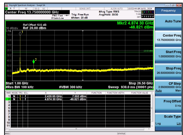
11B-Ant1-2437-1000~26500-PASS
