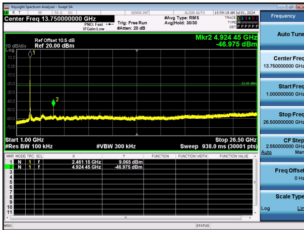
11B-Ant1-2462-1000~26500-PASS
