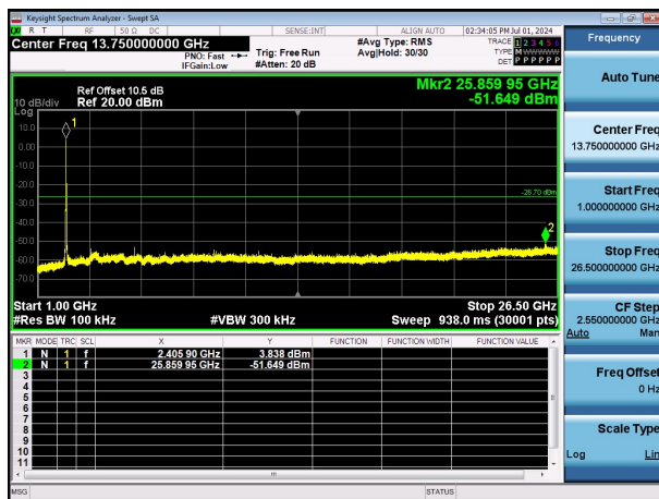
11N20SISO-Ant1-2412-1000~26500-PASS
