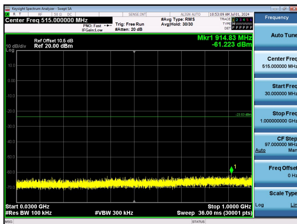
11B-Ant1-2437-30~1000-PASS
