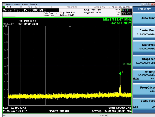
11N20SISO-Ant1-2437-30~1000-PASS
