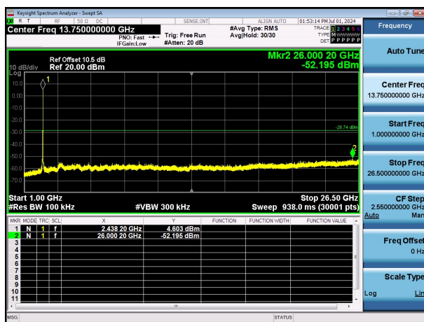
11G-Ant1-2437-1000~26500-PASS
