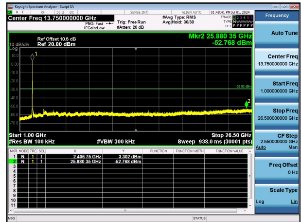
11G-Ant1-2412-1000~26500-PASS
