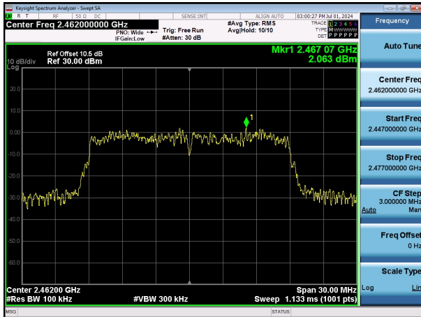
11N20SISO-Ant1-2462-0~Reference-PASS
