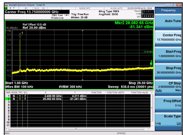
11G-Ant1-2462-1000~26500-PASS
