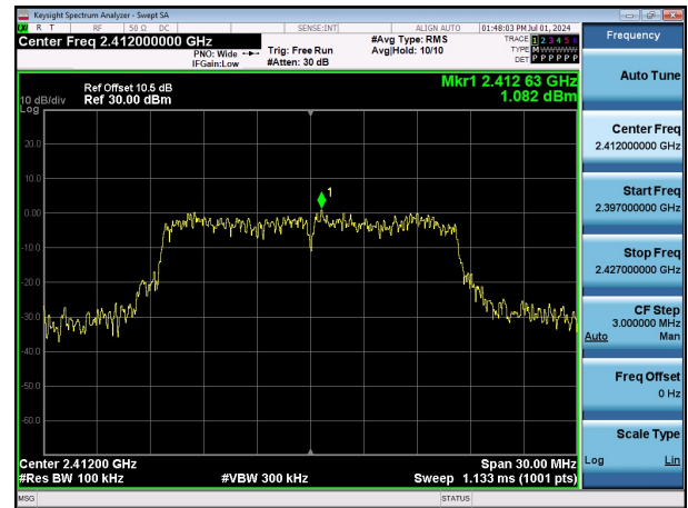
11G-Ant1-2412-0~Reference-PASS
