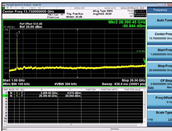
11N20SISO-Ant1-2462-1000~26500-PASS
