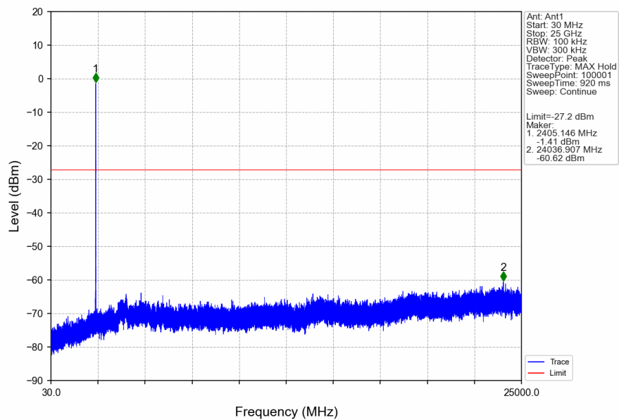
Zigbee_LCH_2405MHz_Ant1_NTNV
