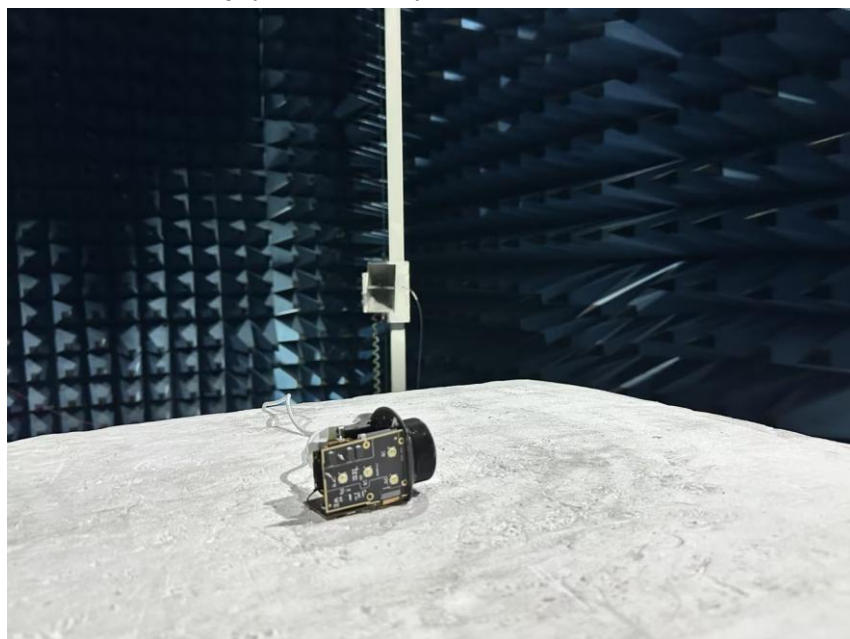
RF Radiated setup (Above 1GHz)
