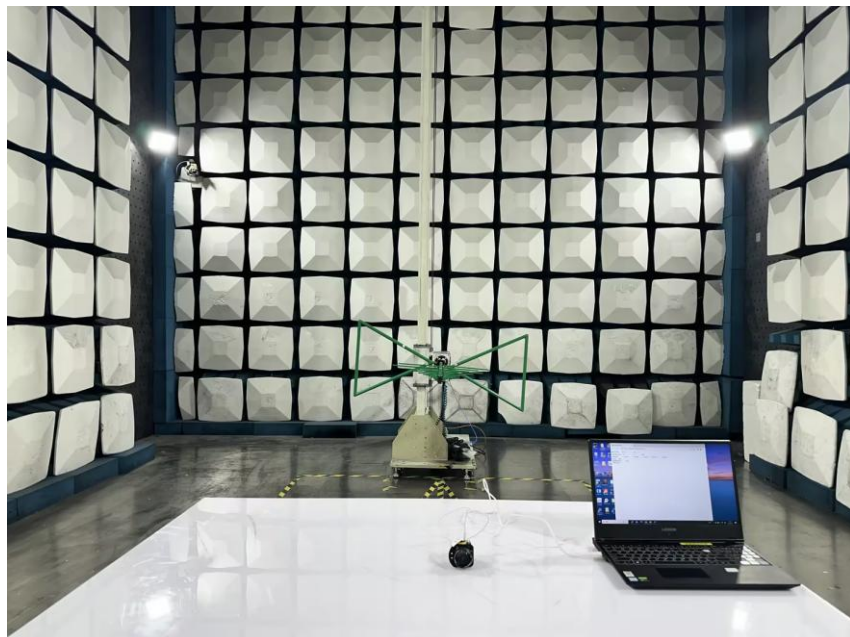
RF Radiated setup (Below 1GHz)
