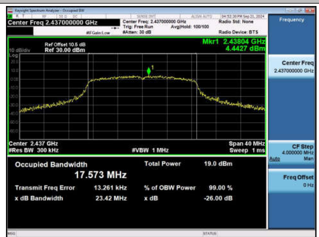
11N20SISO-Ant1-2437
