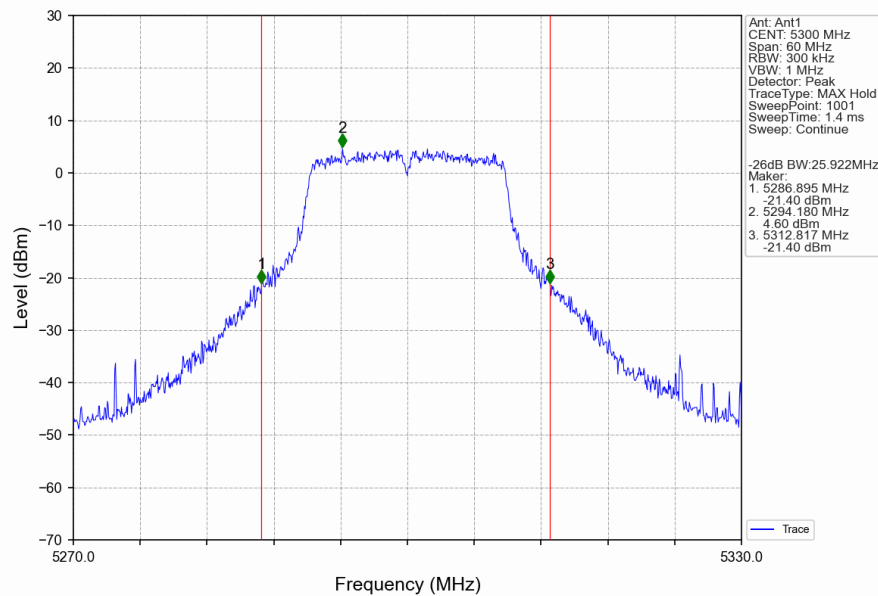
802.11ac(VHT20)_MCH_5300MHz_Ant1_NTNV
