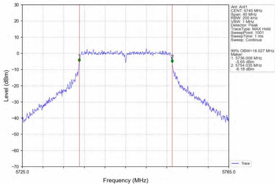
802.11ac(VHT20)_LCH_5745MHz_Ant1_NTNV
