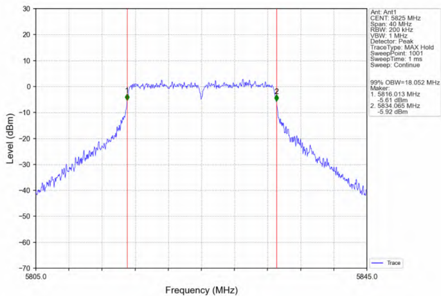
802.11ac(VHT20)_HCH_5825MHz_Ant1_NTNV
