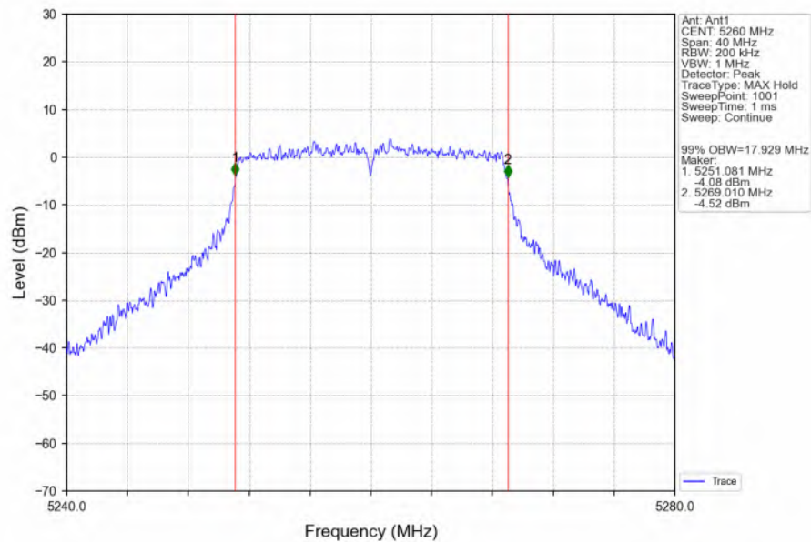
802.11ac(VHT20)_LCH_5260MHz_Ant1_NTNV
