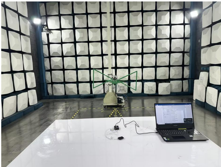
RF Radiated setup (Below 1GHz)
