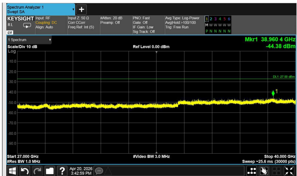
Test_Graph_802.11a_ANT1_5180_6Mbps_Frequency Band 5
