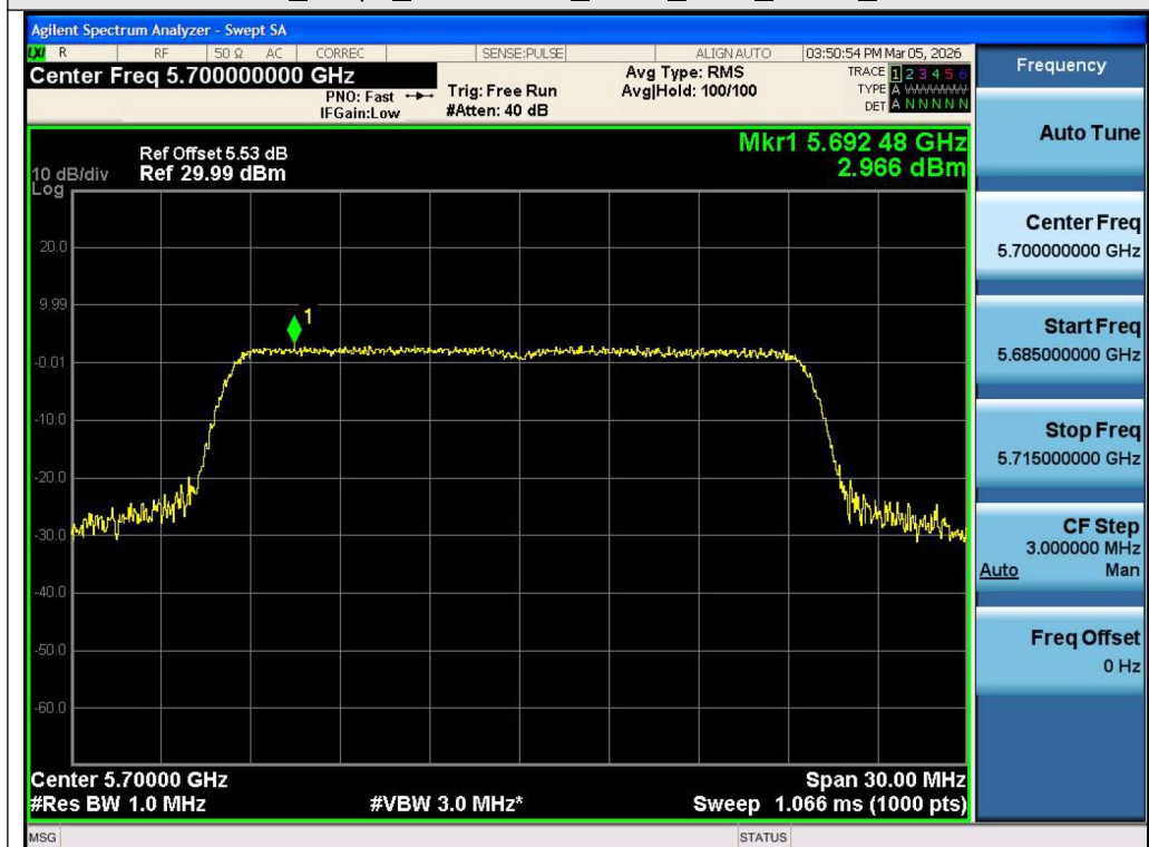
Test_Graph_802.11ax20_ANT1_5700_MCS0_PSD
