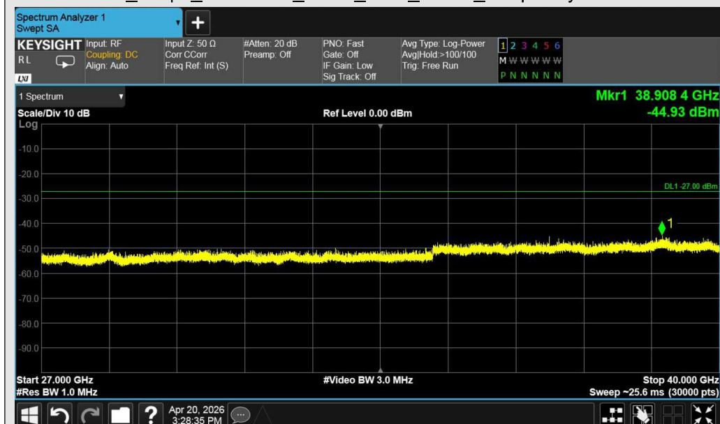
Test_Graph_802.11n40_ANT1_5230_MCS0_Frequency Band 5
