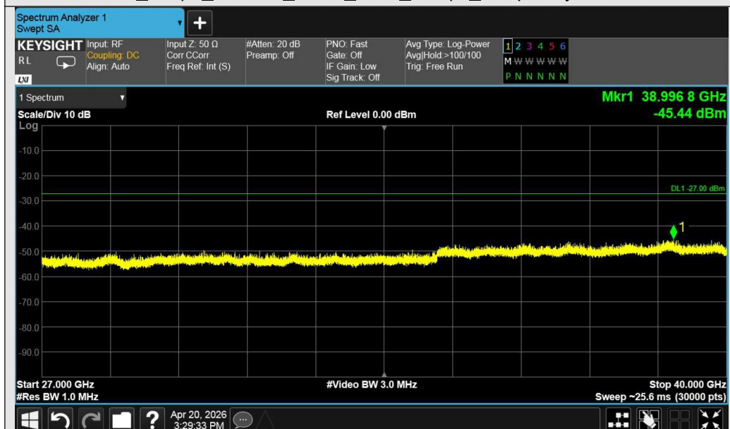
Test_Graph_802.11a_ANT1_5320_6Mbps_Frequency Band 5
