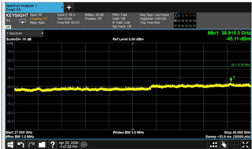
Test_Graph_802.11n40_ANT1_5270_MCS0_Frequency Band 5
