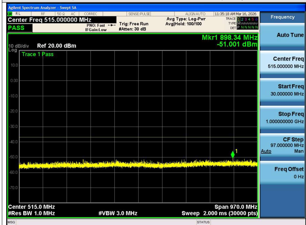
Test_Graph_802.11n40_ANT1_5230_MCS0_Frequency Band 1
