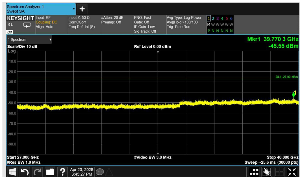
Test_Graph_802.11a_ANT1_5260_6Mbps_Frequency Band 5
