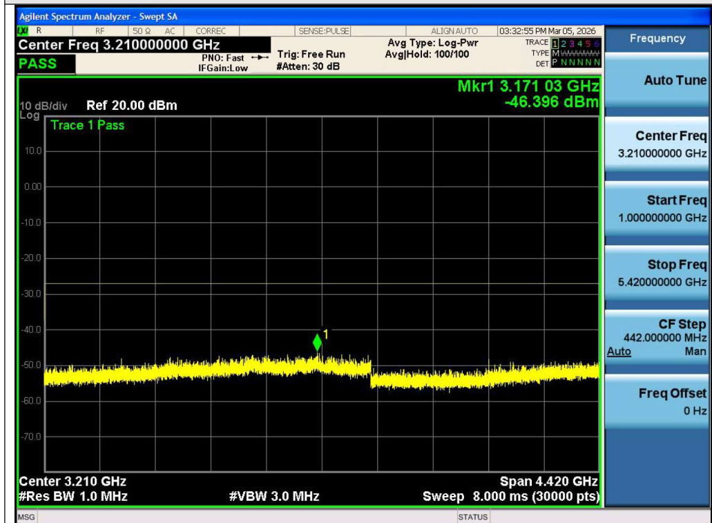
Test_Graph_802.11n40_ANT1_5670_MCS0_Frequency Band 2
