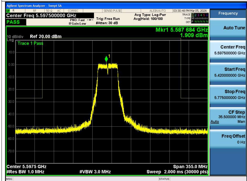
Test_Graph_802.11n40_ANT1_5590_MCS0_Frequency Band 3
