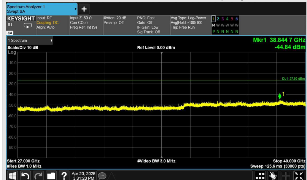
Test_Graph_802.11n40_ANT1_5310_MCS0_Frequency Band 5
