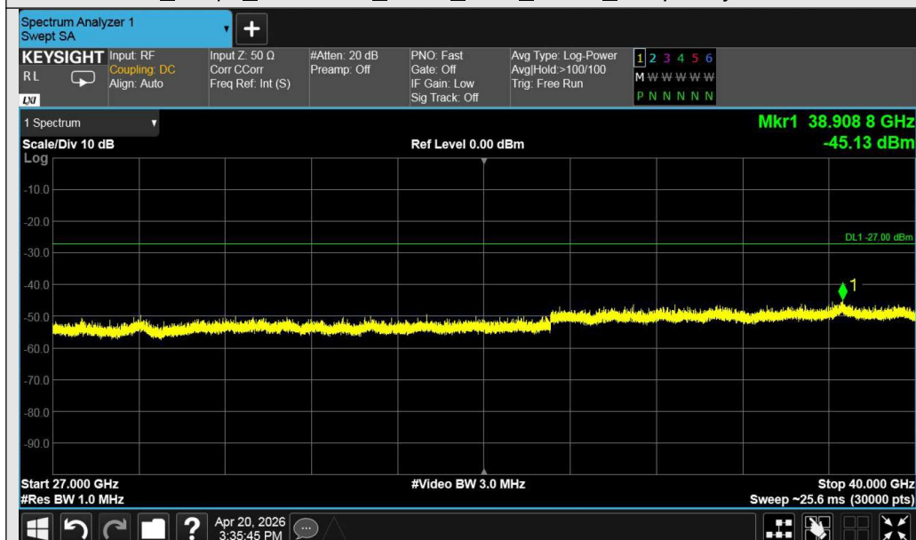
Test_Graph_802.11n40_ANT1_5590_MCS0_Frequency Band 5
