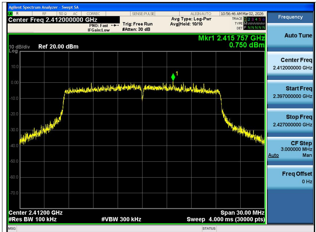
Test_Graph_802.11ax20_ANT1_2412_MCS0_Reference Level
