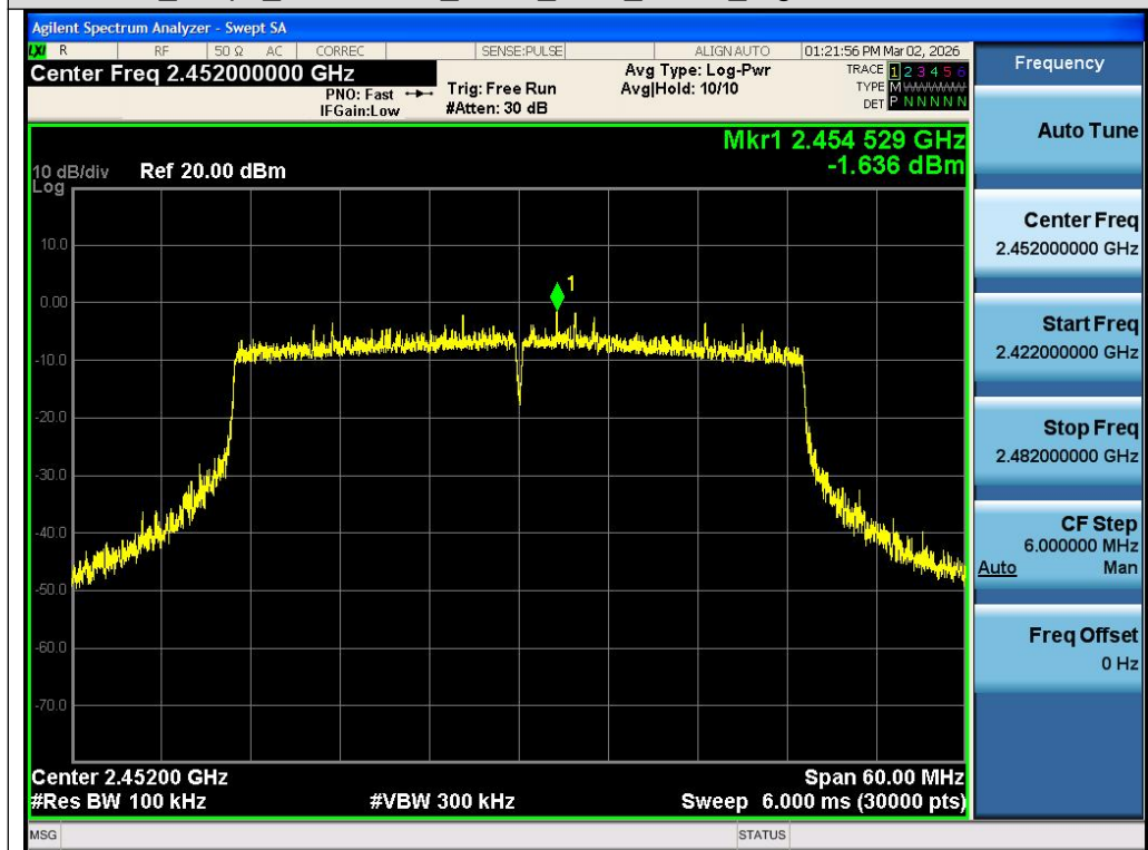
Test_Graph_802.11ax40_ANT1_2452_MCS0_Reference Level
