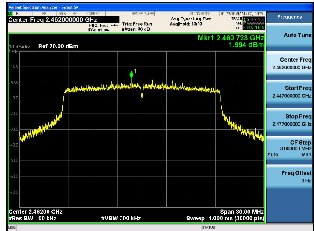
Test_Graph_802.11ax20_ANT1_2462_MCS0_Reference Level
