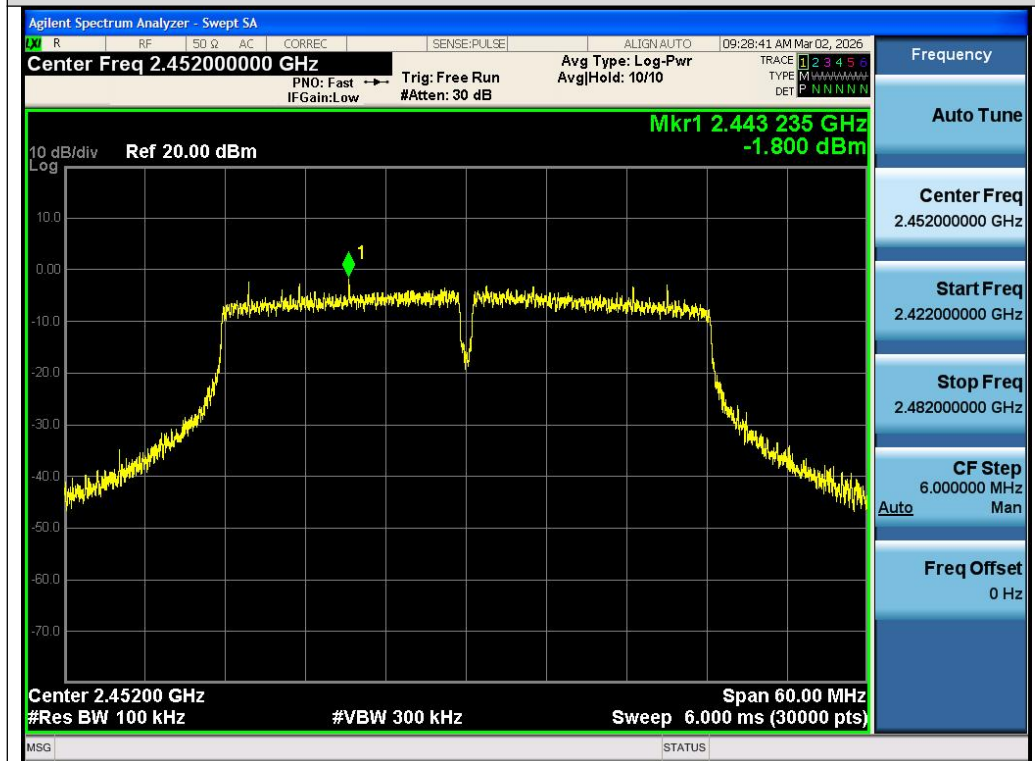
Test_Graph_802.11n40_ANT1_2452_MCS0_Reference Level
