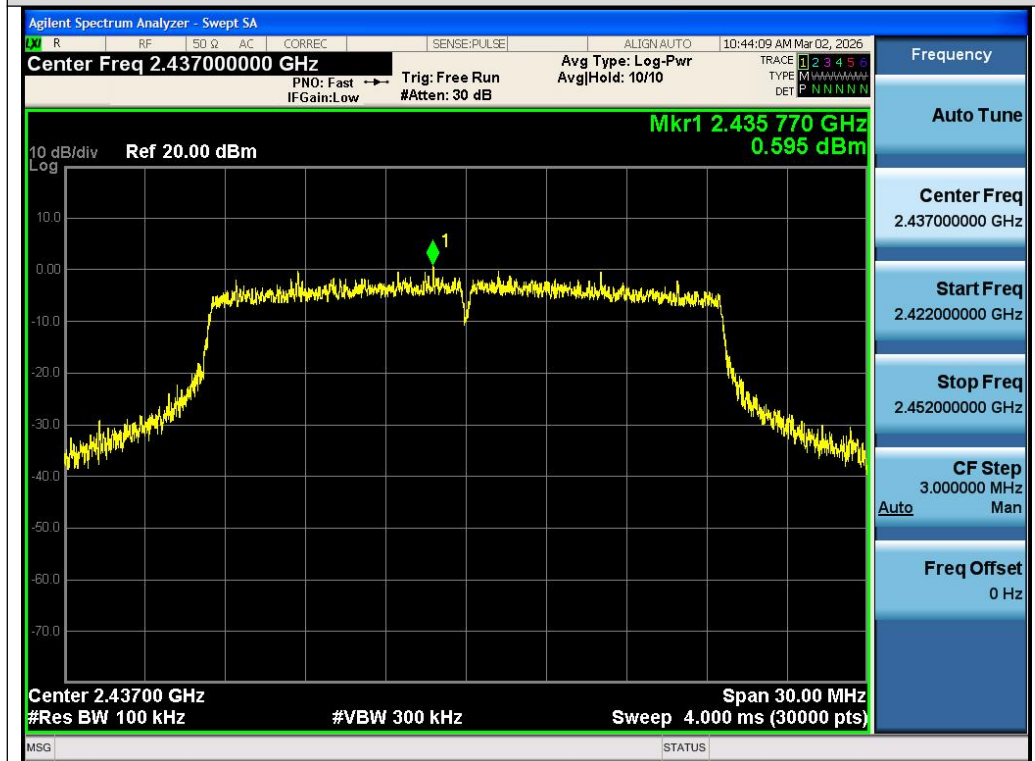
Test_Graph_802.11ax20_ANT1_2437_MCS0_Reference Level
