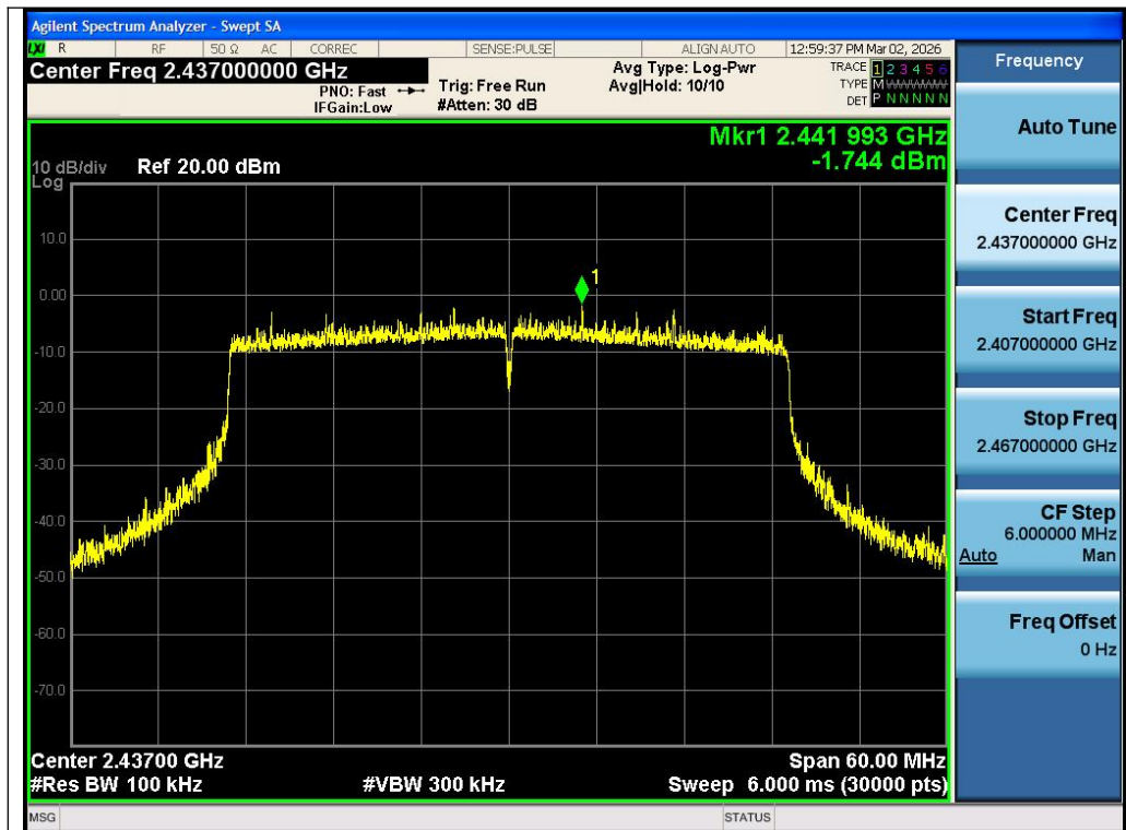
Test_Graph_802.11ax40_ANT1_2437_MCS0_Reference Level
