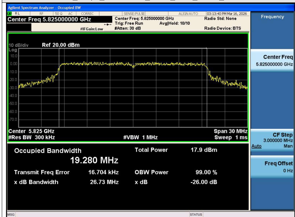
Test_Graph_802.11ax20_ANT1_5825_MCS0_OBW
