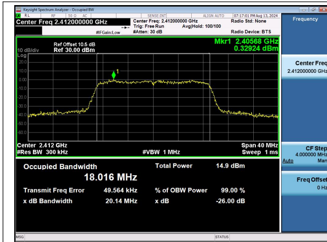
11N20SISO-Ant1-2412
