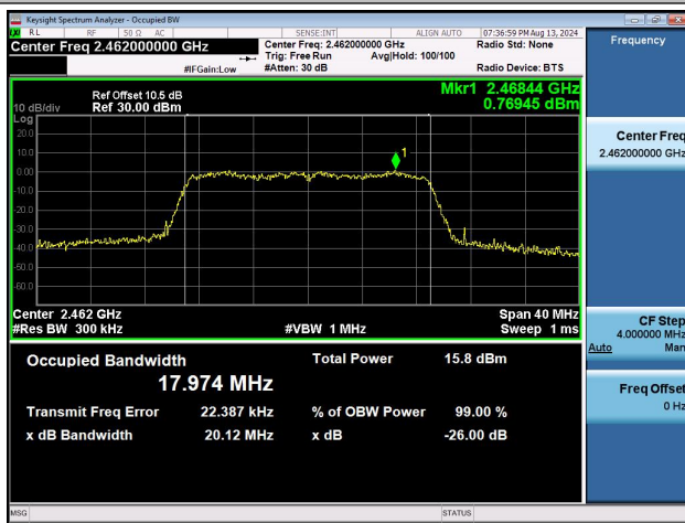
11N20SISO-Ant1-2462
