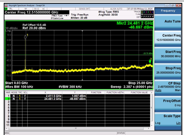
11B-Ant1-2412-30~25000-PASS
