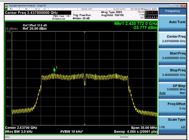
11N20SISO-Ant1-2437-PASS
