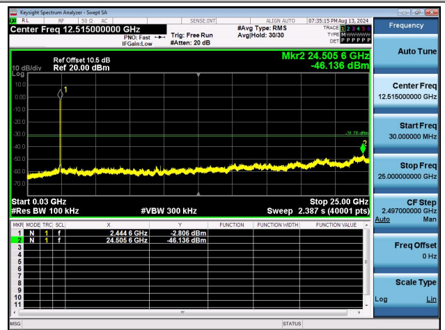
11N20SISO-Ant1-2437-30~25000-PASS
