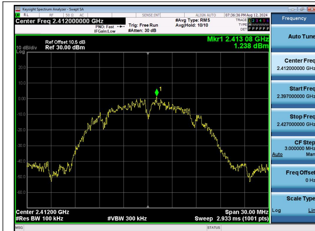
11B-Ant1-2412-0~Reference-PASS
