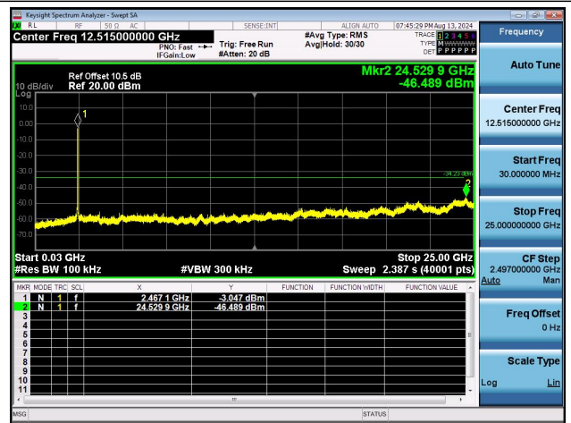
11N20SISO-Ant1-2462-30~25000-PASS
