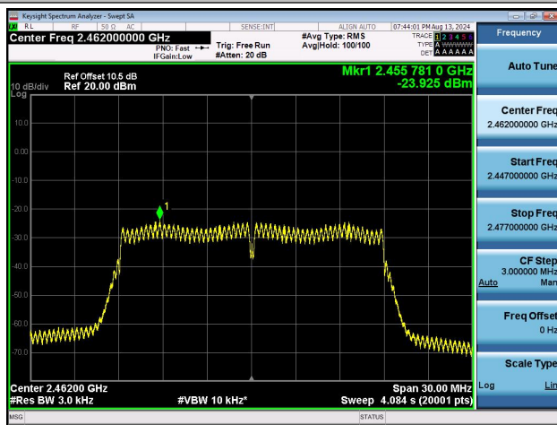
11N20SISO-Ant1-2462-PASS
