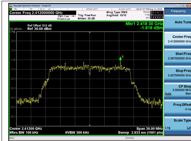
11G-Ant1-2412-0~Reference-PASS
