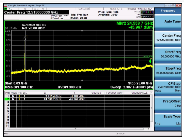
11N20SISO-Ant1-2412-30~25000-PASS
