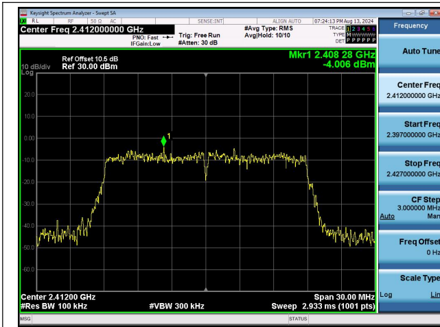
11N20SISO-Ant1-2412-0~Reference-PASS
