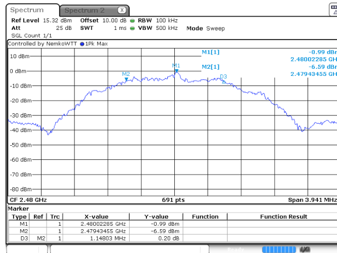
DTS bandwidth, TX 2480 MHz, BW: 2MHz, MOD: GFSK_2Mbps
