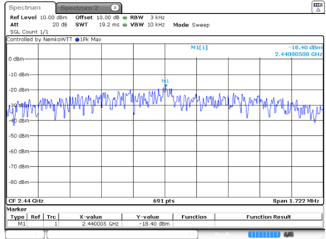
Figure 8.7-5: Power spectral density, GFSK, 2 Mbps, 2440 MHz
