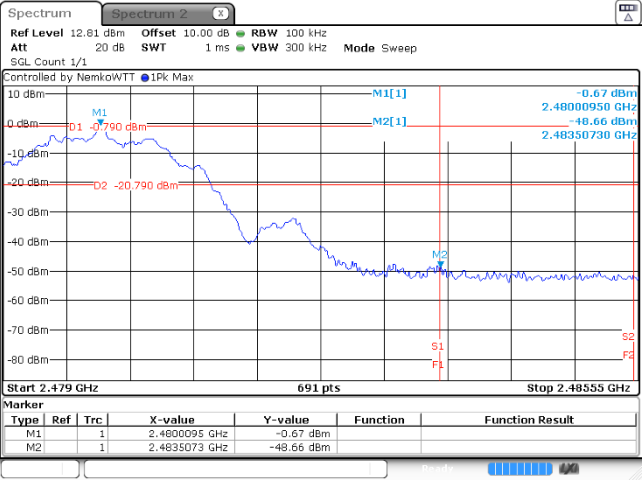
Figure 8.6-4: Authorized band-edge emissions, GFSK, 2 Mbps, 2480 MHz
