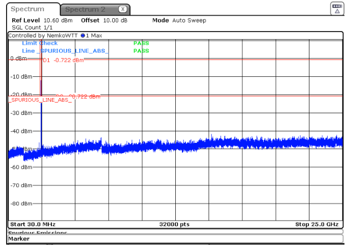
Figure 8.6-10: Antenna port conducted spurious emissions, GFSK, 1 Mbps, 2480 MHz
