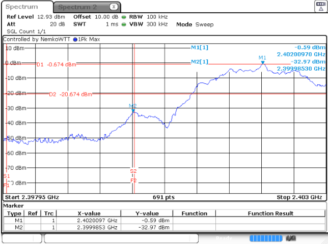
Figure 8.6-3: Authorized band-edge emissions, GFSK, 2 Mbps, 2402 MHz
