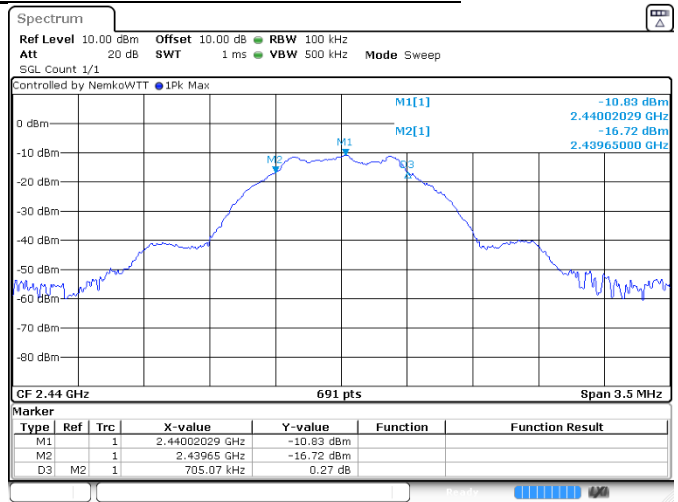
Figure 8.4-2: Minimum 6 dB bandwidth, GFSK, 1 Mbps, 2440 MHz
