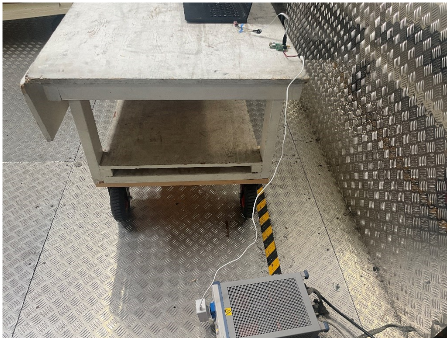
Figure 9 – Test setup, side view.
