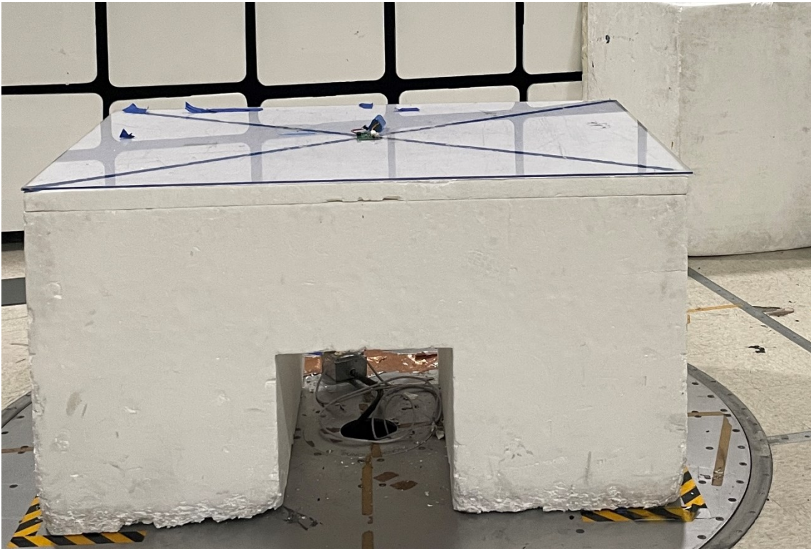
Figure 1 – Test setup
