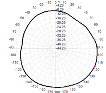
Total(H-XY), Max=-4.26dBi, CirD=9.36
