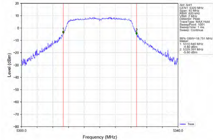
802.11a_HCH_5320MHz_Ant1_NTNV
