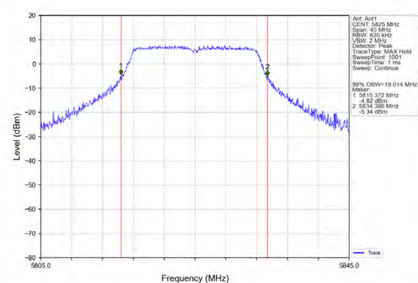
802.11a_HCH_5825MHz_Ant1_NTNV
