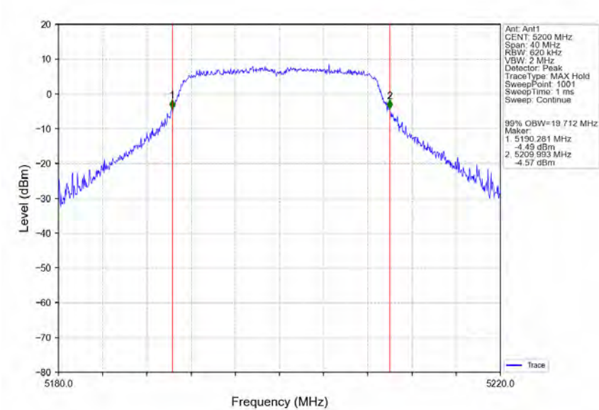
802.11n(HT20)_MCH_5200MHz_Ant1_NTNV
