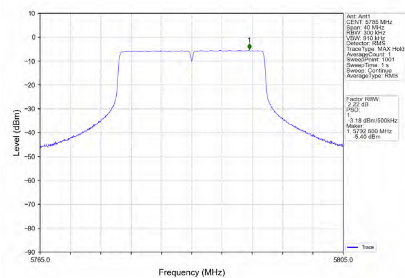
802.11ax(HEW20)_MCH_5785MHz_RU242_Left_Ant1_NTNV
