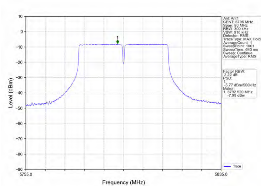
802.11ac(VHT40)_HCH_5795MHz_Ant1_NTNV
