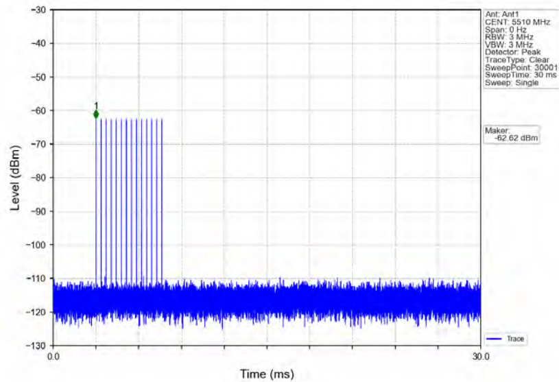
Signal Calibration 802.11ax(HEW40) 2C 5510MHz RadarType5 Trial0
