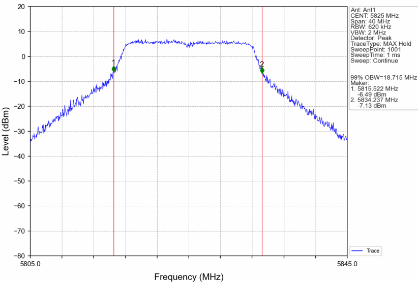
802.11a_HCH_5825MHz_Ant1_NTNV
