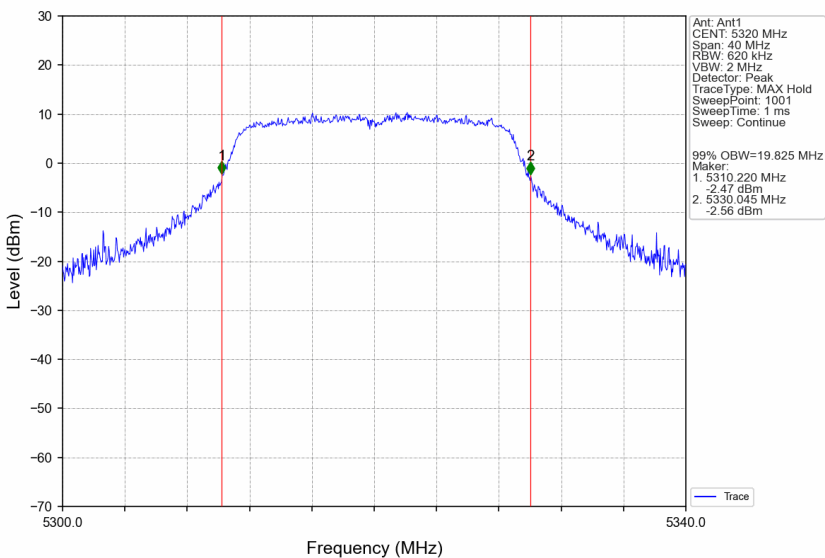
802.11ac(VHT20)_HCH_5320MHz_Ant1_NTNV
