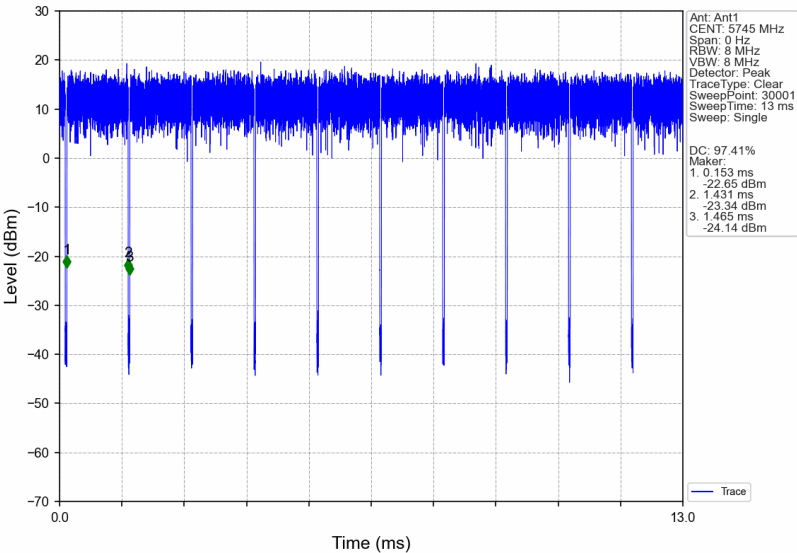
802.11ac(VHT20)_LCH_5745MHz_Ant1_NTNV
