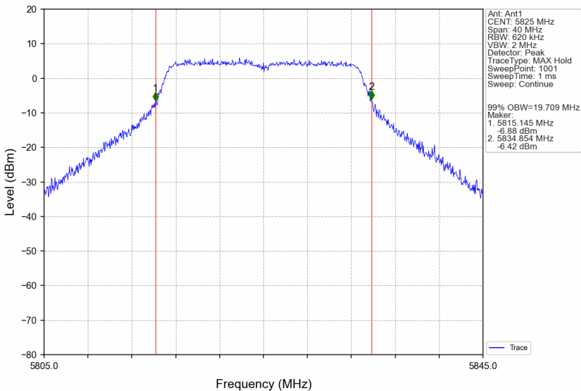
802.11ac(VHT20)_HCH_5825MHz_Ant1_NTNV
