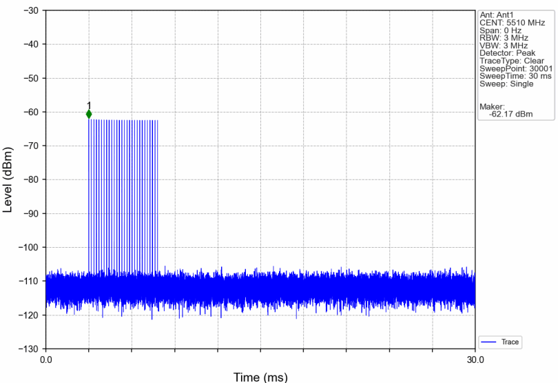
Signal Calibration 802.11ax(HEW40) 2C 5510MHz RadarType2 Trial0
