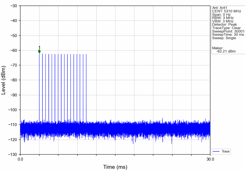
Signal Calibration 802.11ax(HEW40) 2A 5310MHz RadarType4 Trial0
