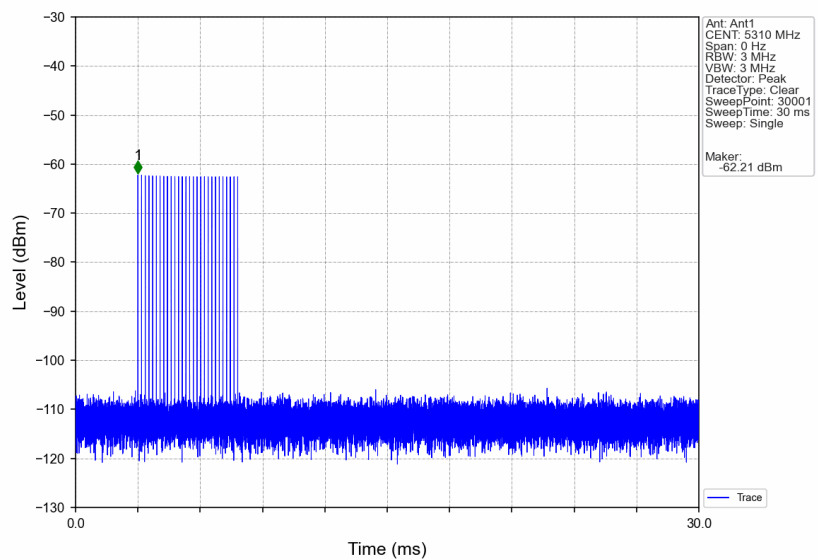
Signal Calibration 802.11ax(HEW40) 2A 5310MHz RadarType2 Trial0
