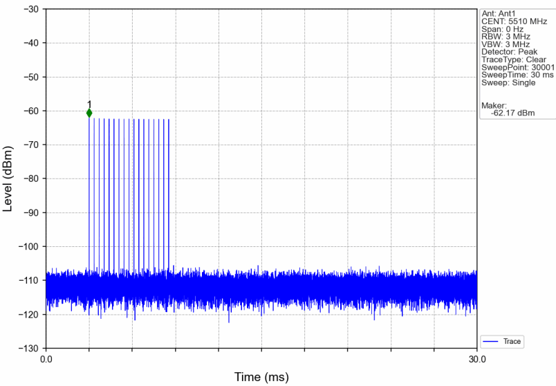
Signal Calibration 802.11ax(HEW40) 2C 5510MHz_RadarType4_Trial0
