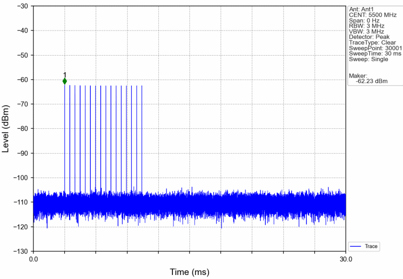
Signal Calibration 802.11ax(HEW20) 2C 5500MHz RadarType5 Trial0
