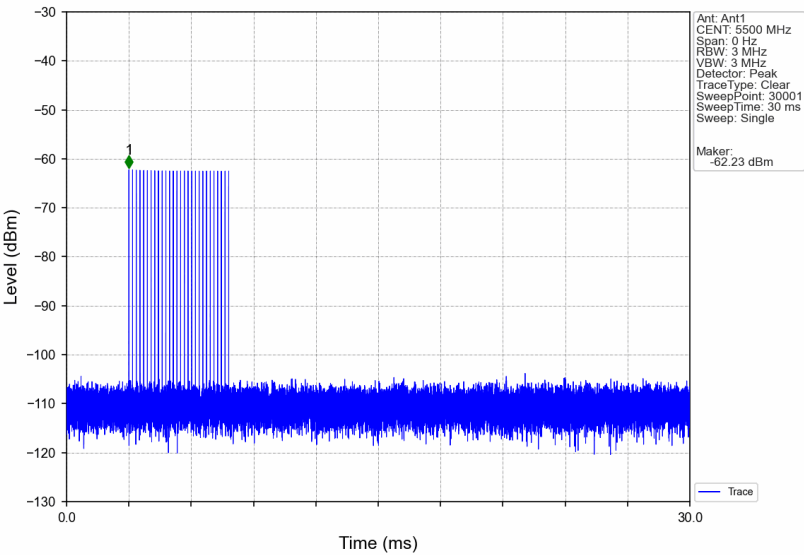
Signal Calibration 802.11ax(HEW20) 2C 5500MHz RadarType3 Trial0
