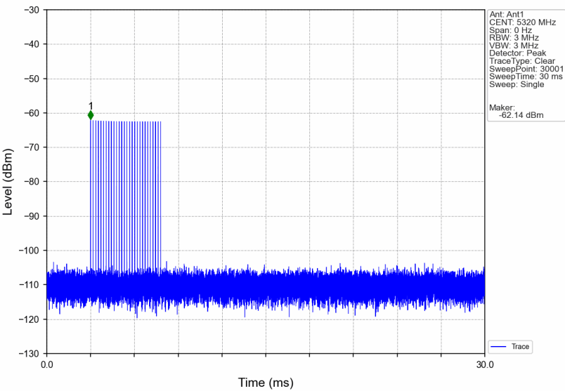
Signal Calibration 802.11ax(HEW20) 2A 5320MHz RadarType3 Trial0
