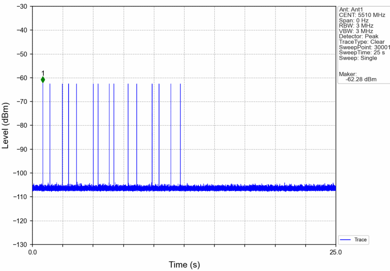
Signal Calibration 802.11ax(HEW40) 2C 5510MHz_RadarType6_Trial0
