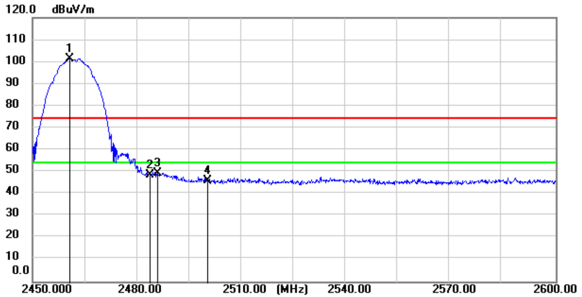
11b_TX_CH_11_Vertical_Peak
