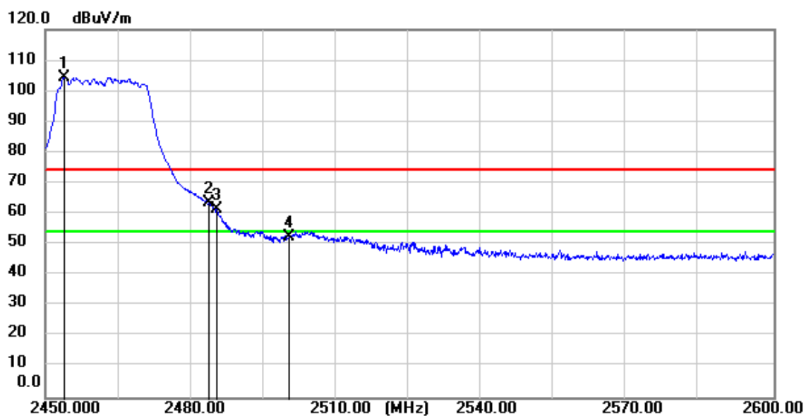
11(HE20)_TX_CH_11_Vertical_Peak
