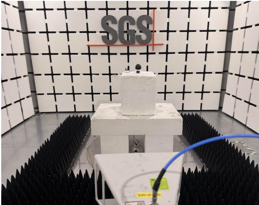
RF Radiated Setup (Above 1GHz)
