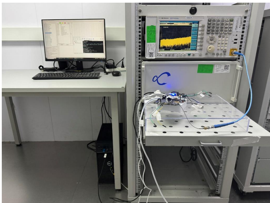
Conducted Test-Wi-SUN 2
