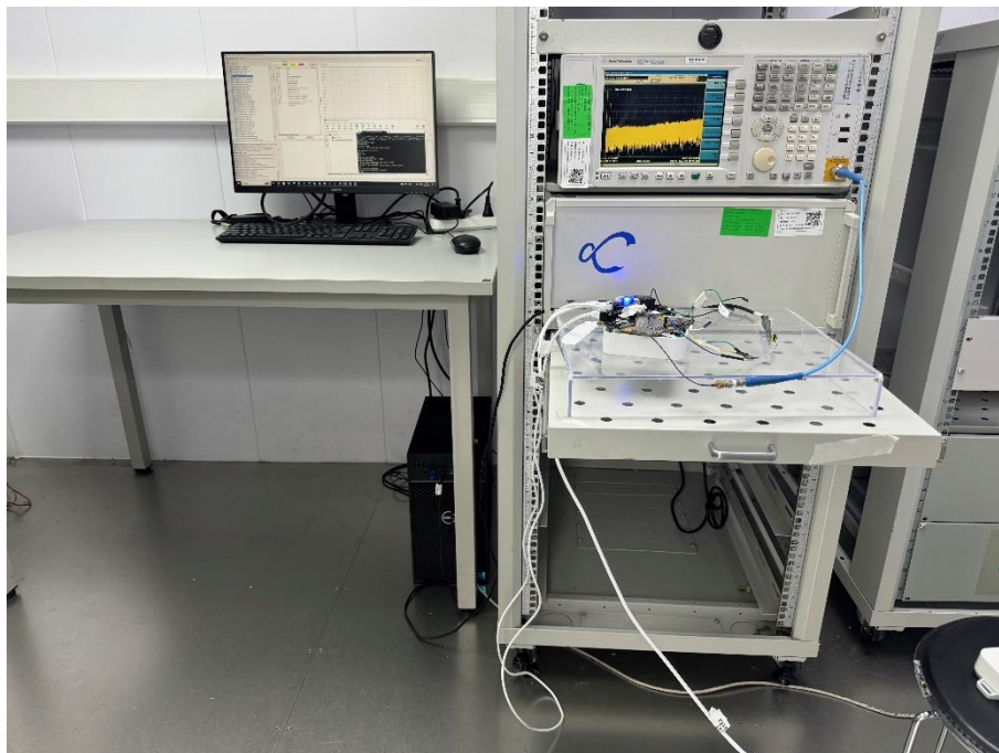
Conducted Test-Wi-SUN 1
