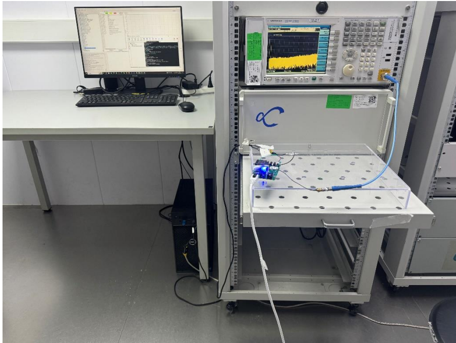
Conducted Test-Wi-SUN
