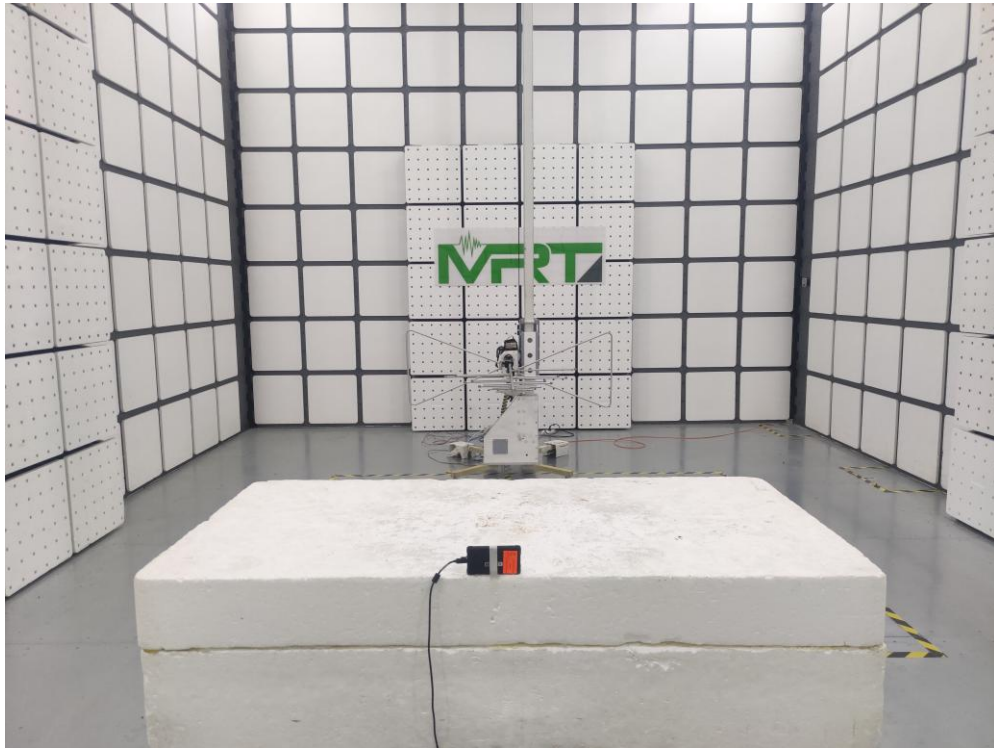
Description: Radiated Emissions Test Setup for 1 ~ 18GHz
