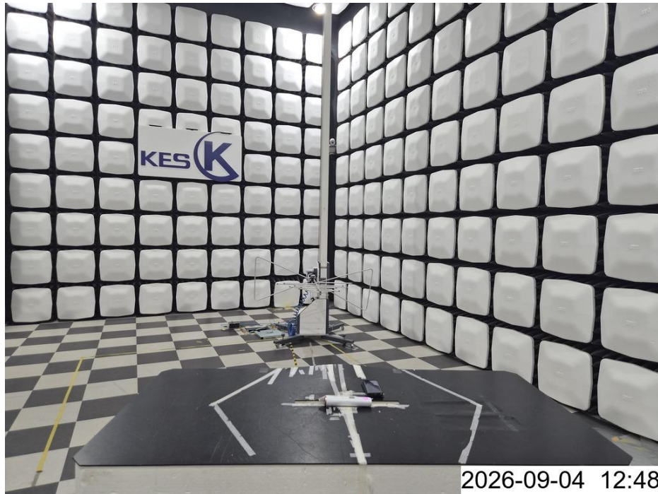
<Radiated Emissions(Below 1 GHz) - Front> mode 3
