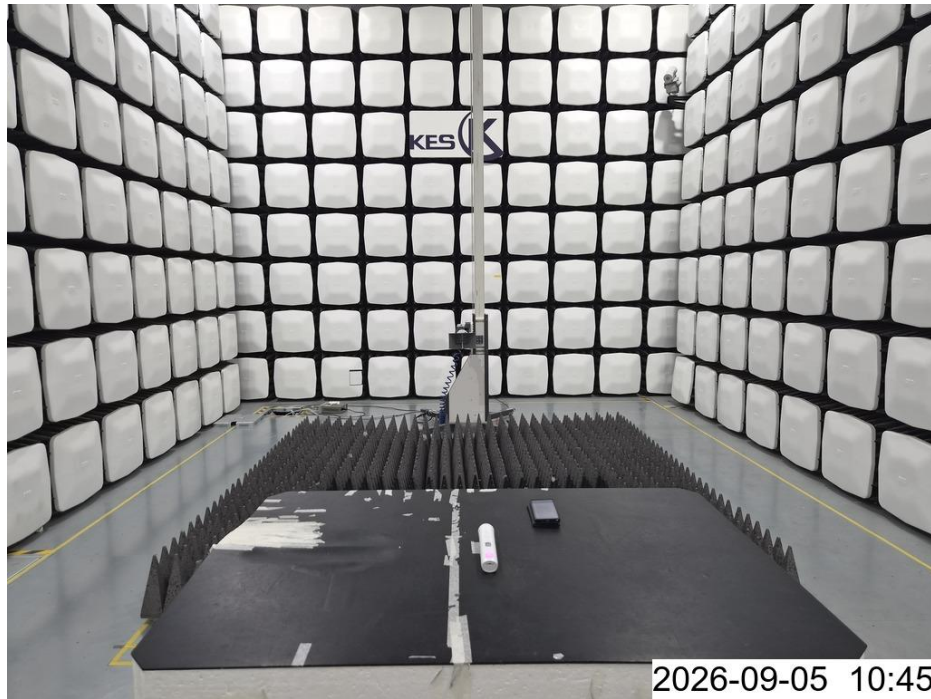
<Radiated Emissions(Above 1 GHz) - Front> mode 3
