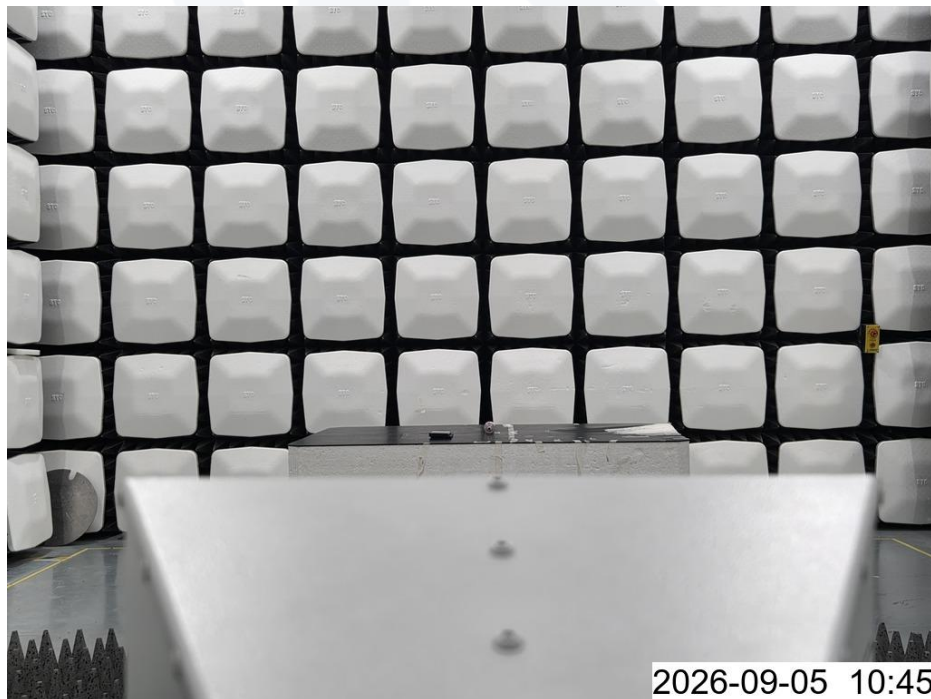
<Radiated Emissions(Above 1 GHz) - Rear> mode 3
