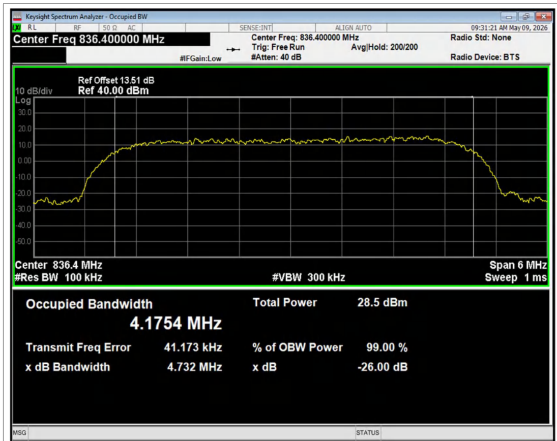
HSDPA Band5 Channel=4182 NVNT
