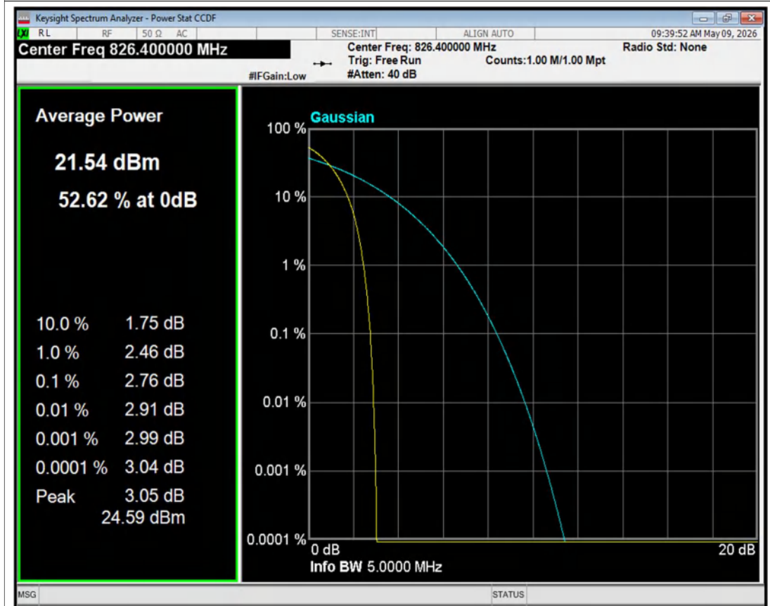
HSUPA Band5 Channel=4132 NVNT
