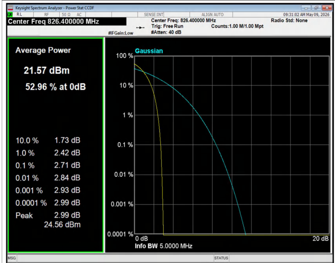
HSDPA Band5 Channel=4132 NVNT
