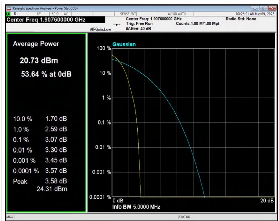
HSDPA Band2 Channel=9538 NVNT
