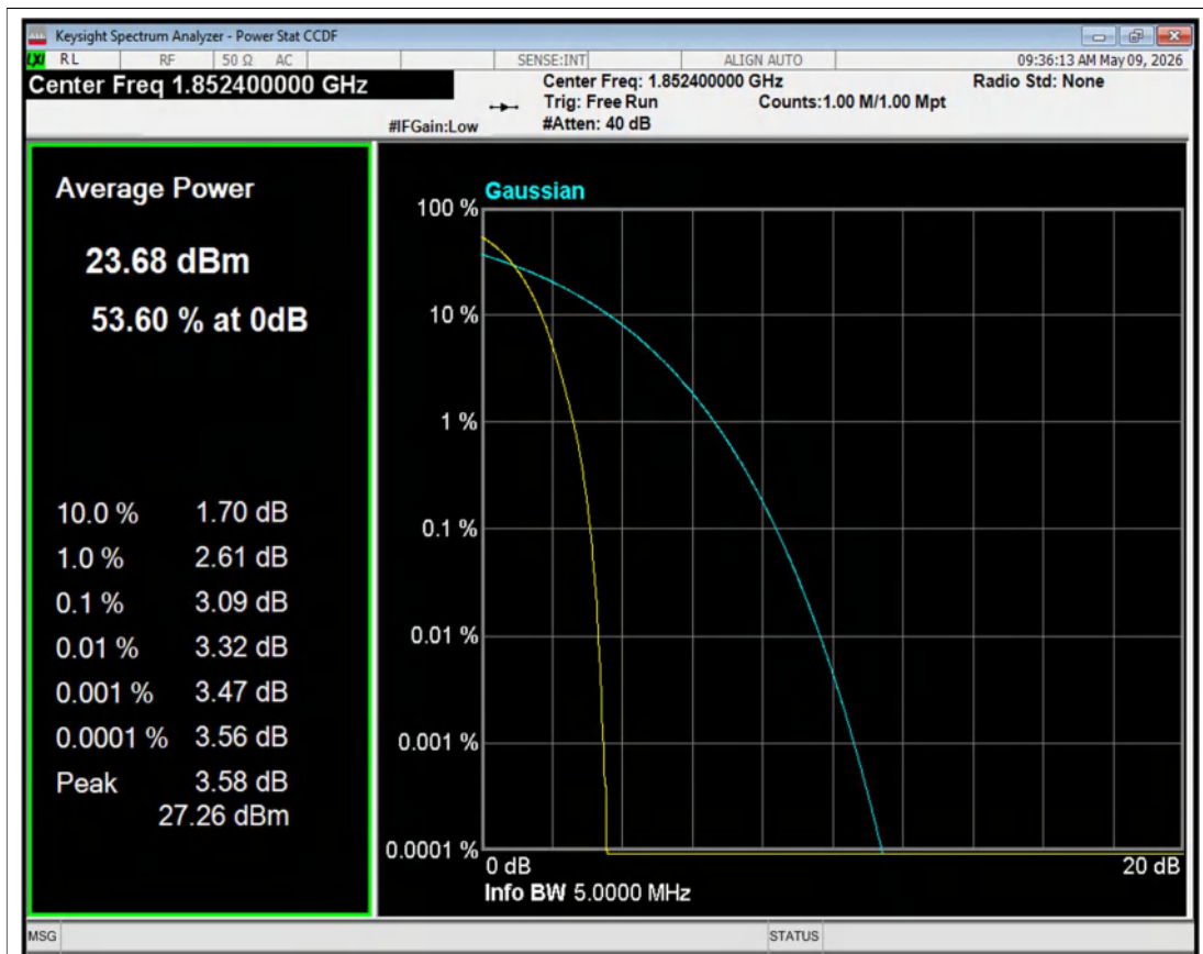
HSUPA Band2 Channel=9262 NVNT
