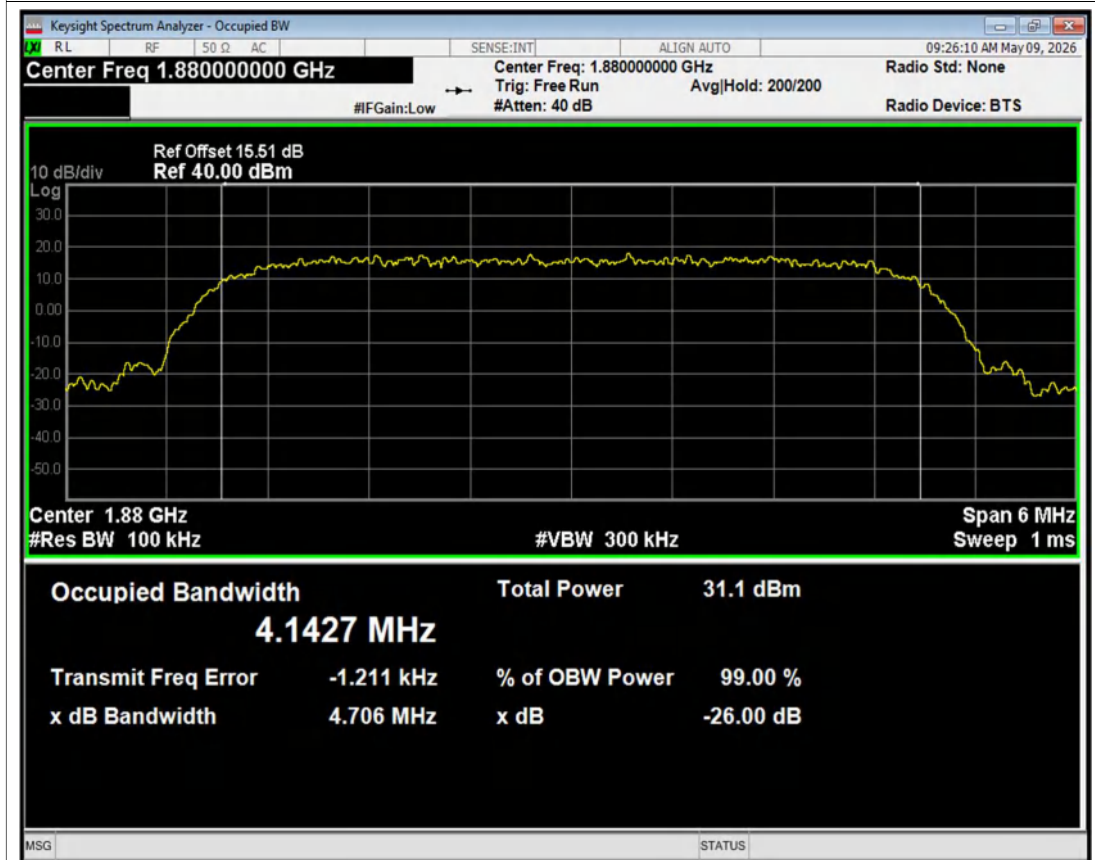
HSDPA Band2 Channel=9400 NVNT
