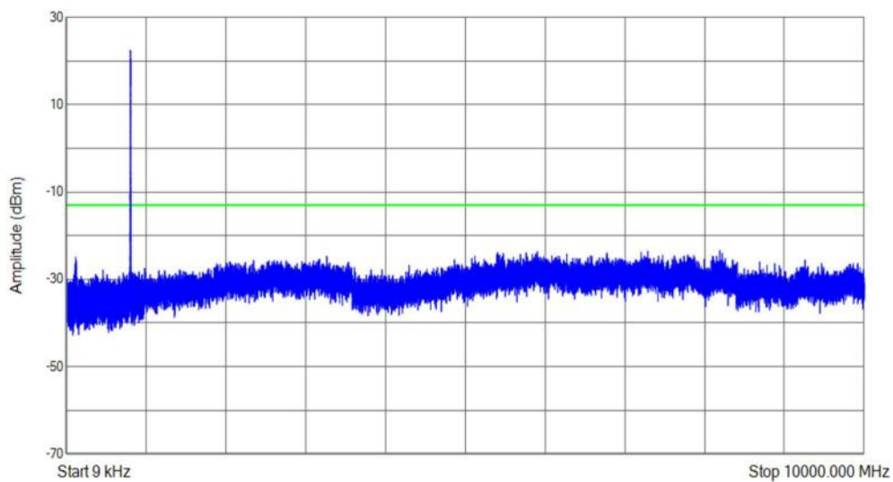
HSDPA Band2 Channel=9538 NVNT
