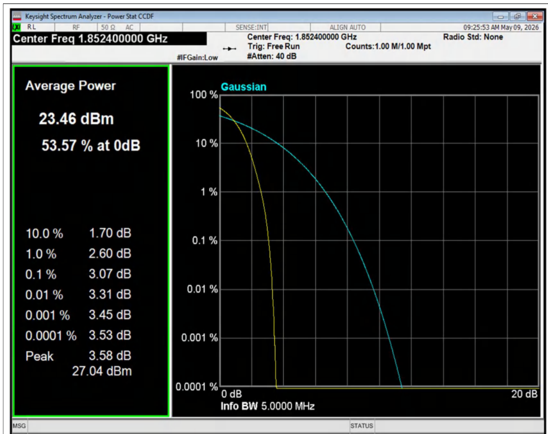
HSDPA Band2 Channel=9262 NVNT
