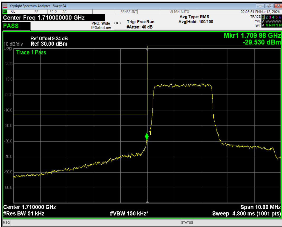
Band66 QPSK BW=5MHz Channel=131997 RB Size=12 Position=#Max
