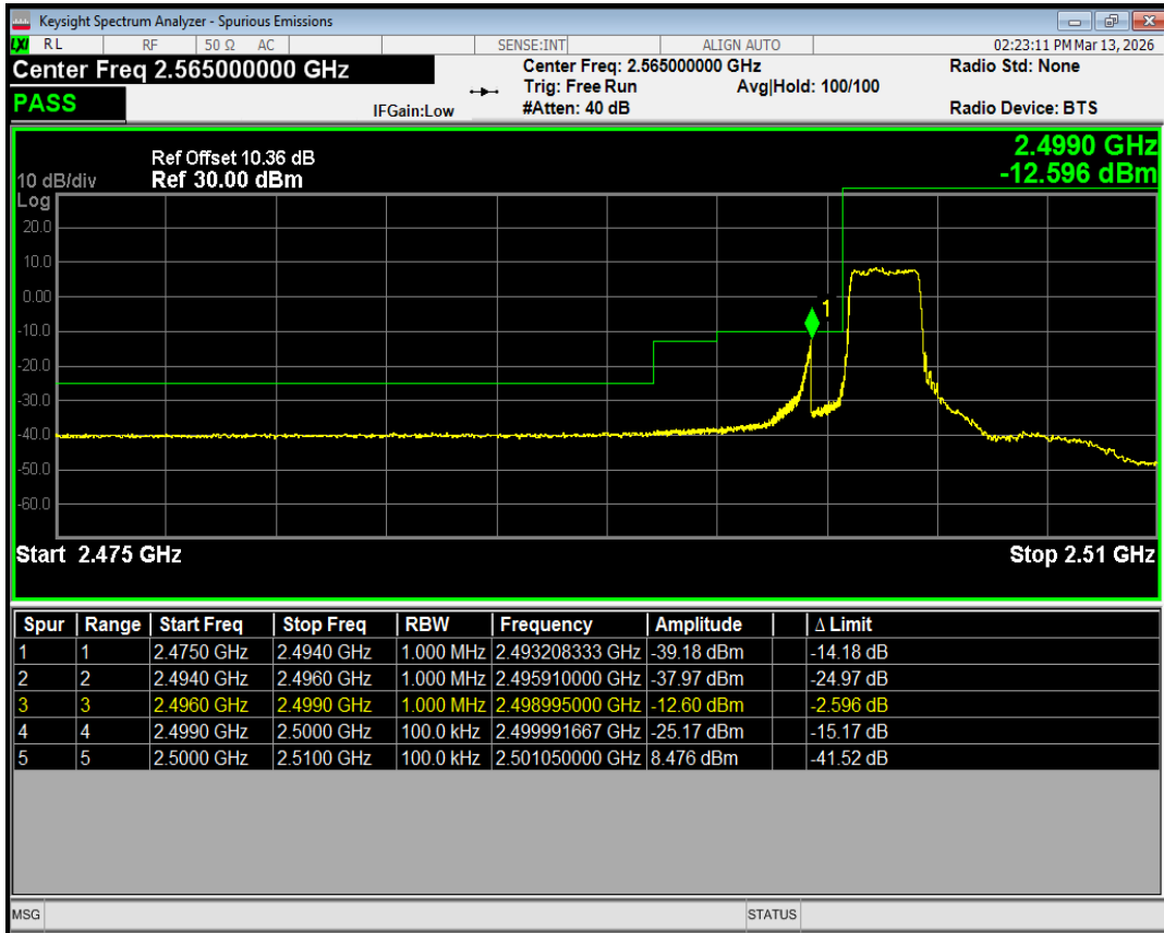
Band7 QPSK BW=5MHz Channel=20775 RB Size=12 Position=#Max
