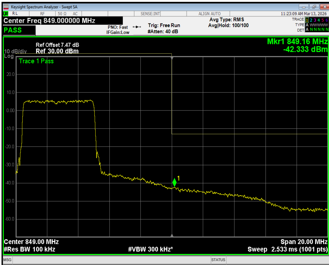
Band5 QAM16 BW=10MHz Channel=20600 RB Size=25 Position=#Max
