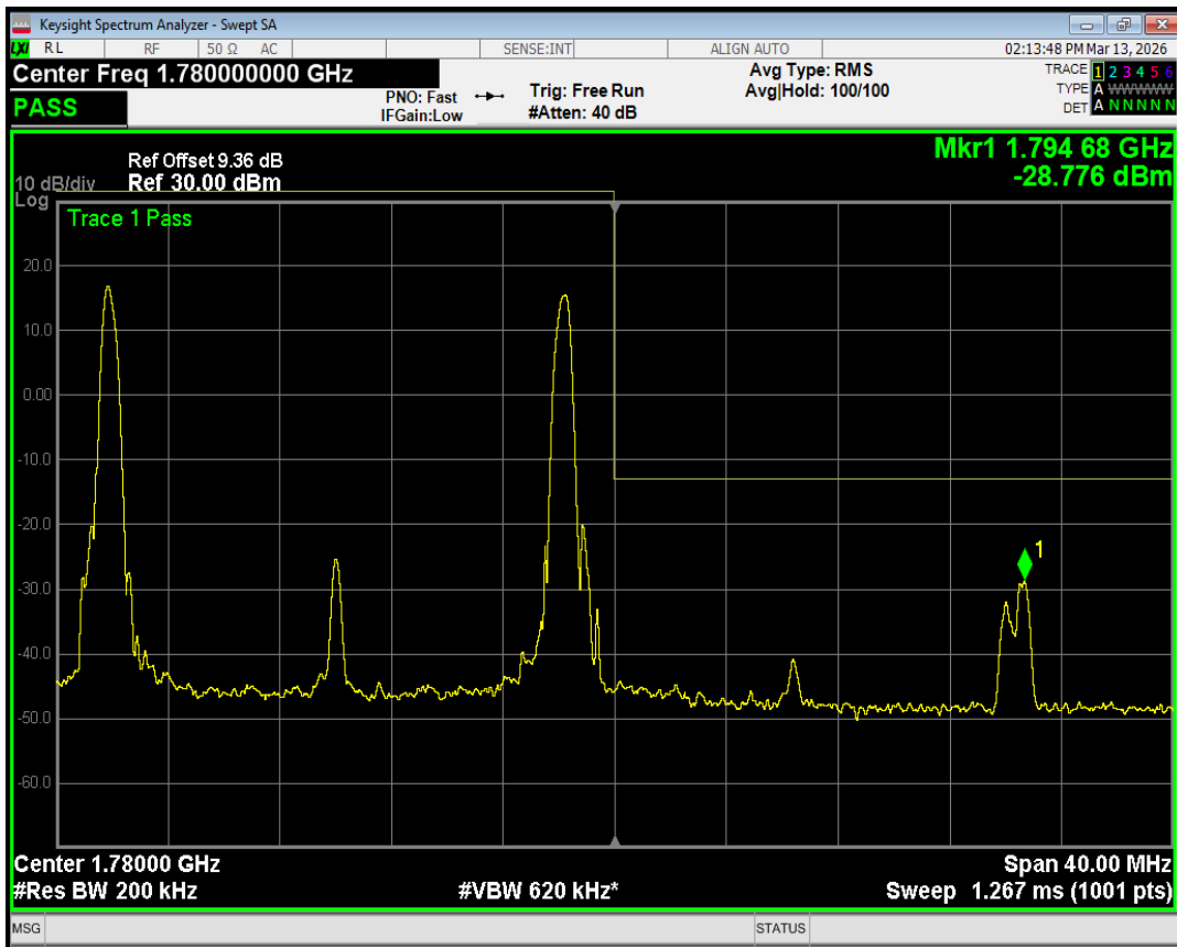
Band66 QAM16 BW=20MHz Channel=132572 RB Size=50 Position=#Max
